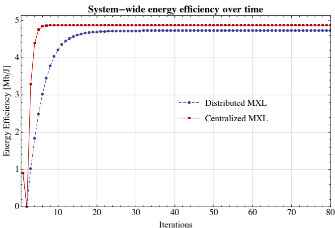
Fig. 4. Unilateral versus system-wide energy efficiency maximization.
