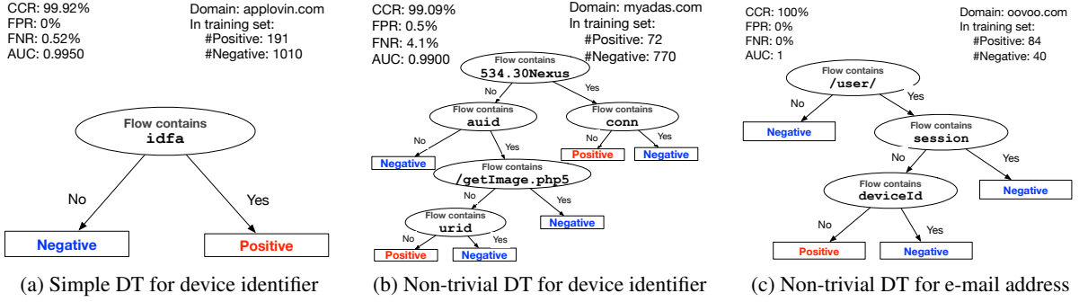
Figure 4: Example decision trees (DTs) for ReCon’s per-domain per-OS classifiers. The classifier beings at the root (top) node, and traverses the tree based on whether the term at each node is present. The leaves (boxes) indicate whether there is a PII leak (positive) or not (negative) for each path. The top right of each figure shows the number of positive/negative samples used to train each DT.
