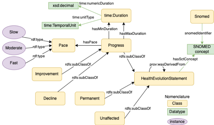
Fig. 1: HECON Ontology core concepts.
