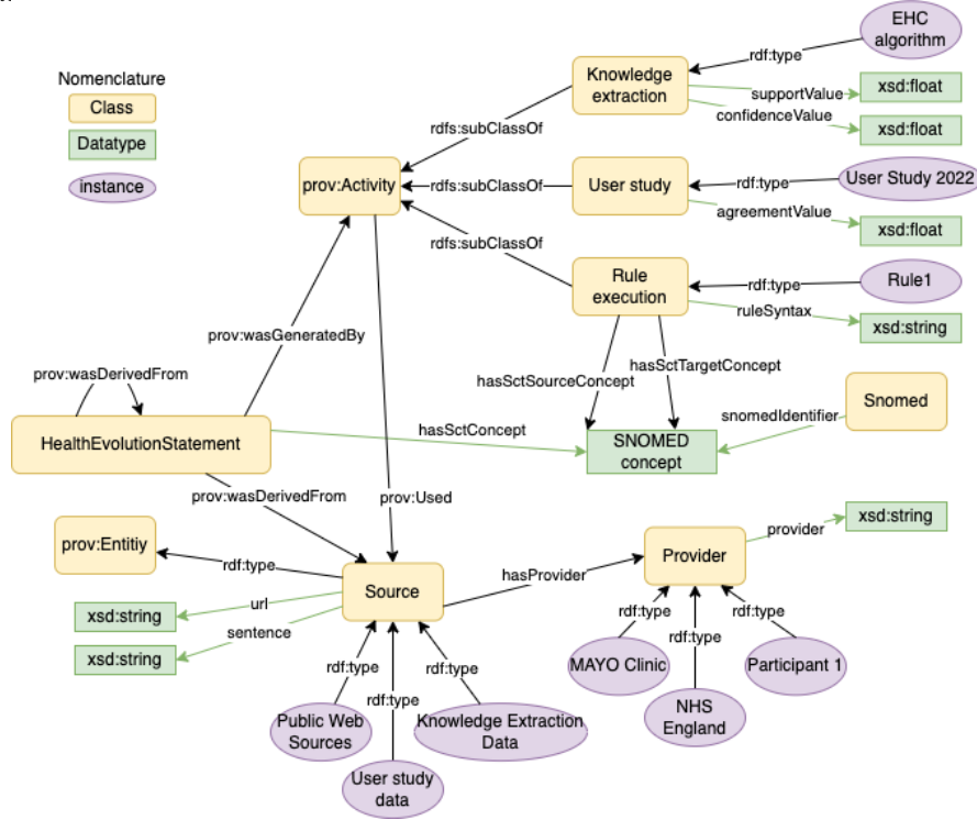
Fig. 2: HECON Ontology provenance representation.
