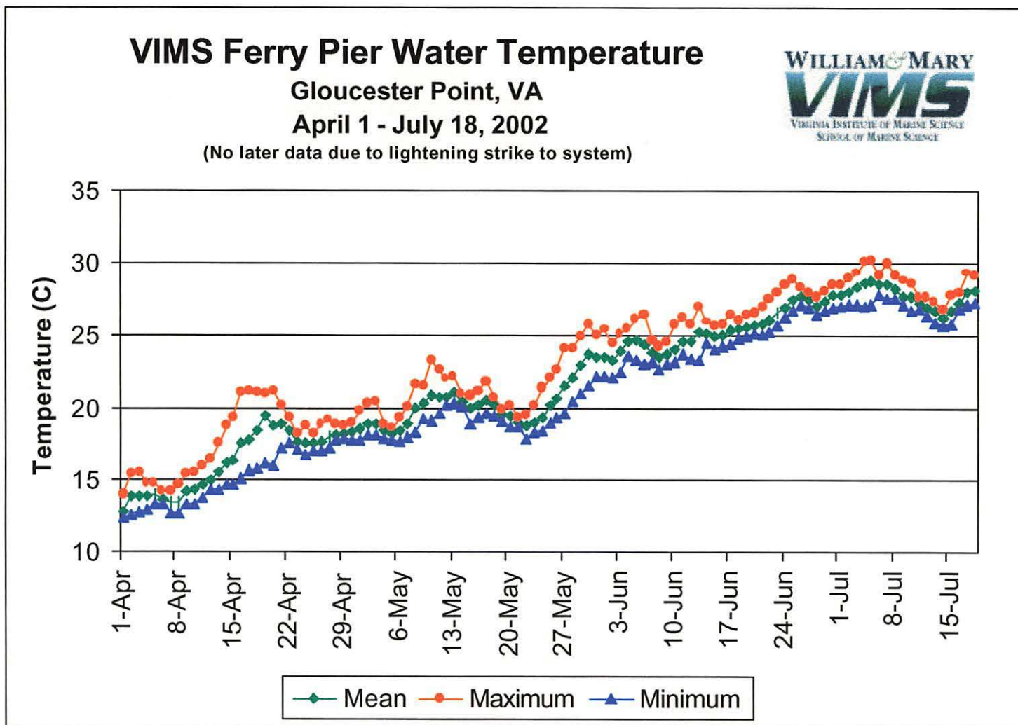
Figure 7. Gloucester Point, VA sea surface temperatures as recorded at the VIMS Ferry Pier from April 1 – July 18. Data acquired from the VIMS Meteorological and Hydrographic Online Archives at http://www.vims.edu/resources/databases.html#pier .
