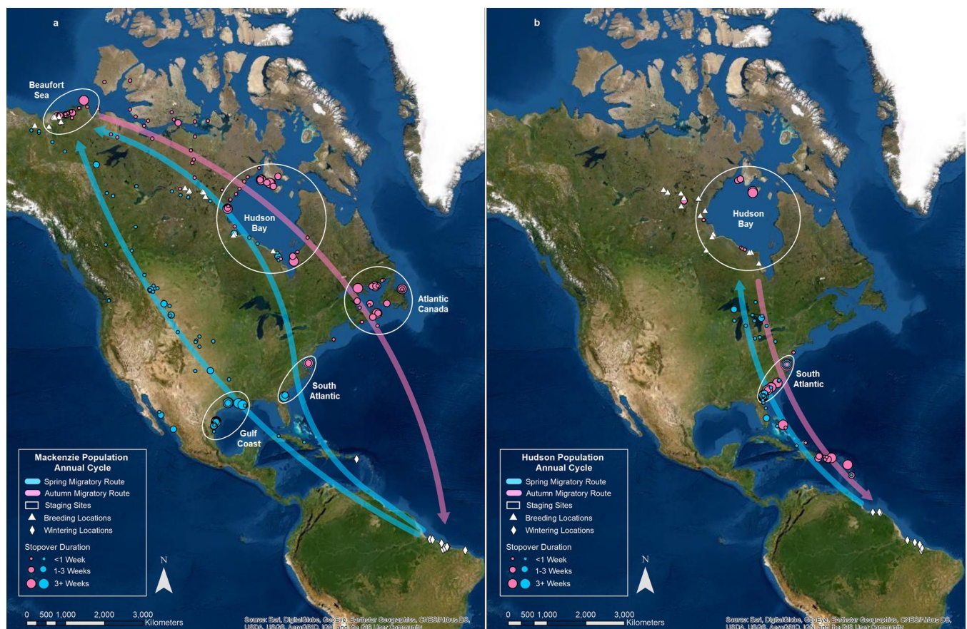
Fig 1. Stylized, Composite Maps of The Annual Cycle for the Mackenzie Delta (1a) and the Hudson Bay (1b) Whimbrel Populations. Information represents a synthesis of multiple years of tracking data. Dots and diamonds represent centroids of locations from periods when birds were not flying. Figure was created by one of the authors using ArcGIS 10.4.1. Basemap provided by: ESRI, Digital Globe, GeoEye, Earthstar Geographics, CNES/Airbus DS, USDA, USGS, AeroGRID, IGN, and the GIS User Community.
