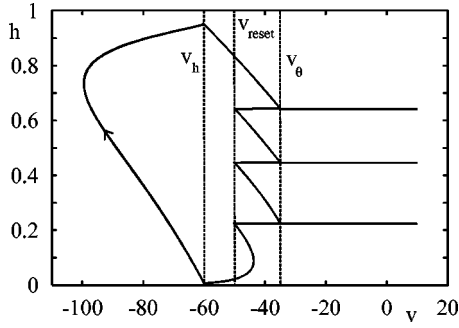
FIG. 3. A 3:1 bursting orbit, I_0 = -0.5 , I_1 = 1 , and f = 2.5 .
