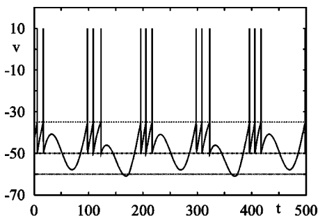
FIG. 10. A 6:2 state at (I_0, I_1) = (2.3, 1.3) .
