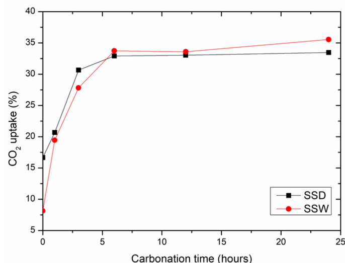
Figure 3. The effect of carbonation time on \text{CO}_2 uptake of compacts made from the SSD and SSW. The standard deviations of \text{CO}_2 uptake ranged from 0.26% to 1.28%.
