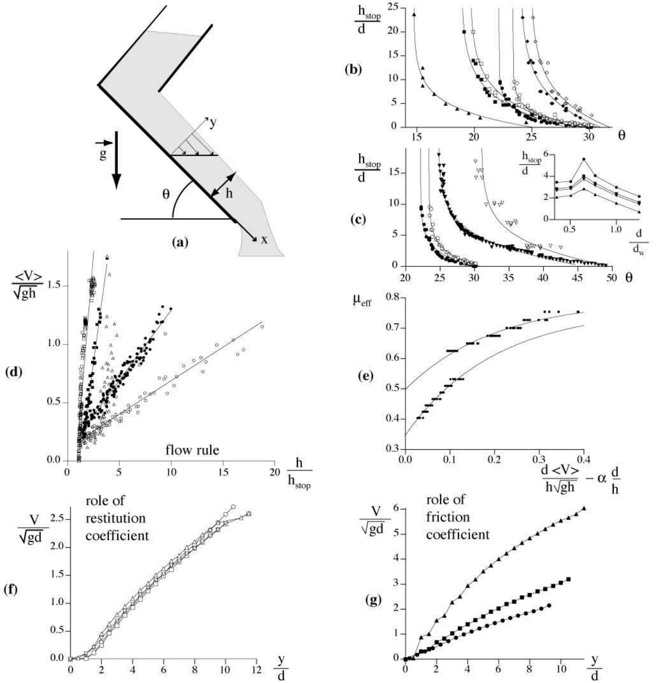
Fig. 5. Rough inclined plane. (a) Set up. (b) h_{\text{stop}}(\theta) (black symbols) and h_{\text{start}}(\theta) (white symbols) from simulations IP3 (▲), experiments IP5 with glass beads (○, ●), IP6 with mustard seeds (◇, ◆) or with glass beads on carpet (□, ■). See text for the fit. (c) Same as (b) for experiments IP5 with glass beads (○, ●), IP7 with glass beads on velvet (▽, ▼). Inset: h_{\text{stop}} for different roughness condition from experiment IP8 \theta = 27^\circ (●), \theta = 28^\circ (■), \theta = 28.3^\circ (▼), \theta = 30^\circ (▲). (d) Froude number \langle V \rangle / \sqrt{gh} as a function of h/h_{\text{stop}}(\theta) from simulation IP3 (○), experiments IP5 with glass beads on glass beads (●), sand on sand (□), IP6 sand on moquet (■), IP7 glass beads on velvet (△). Lines are fits by eq. (7). (e) Effective friction deduced from the flow rule (see text). Experiment IP5 with glass beads (●), with sand (■). Continuous lines are deduced from eq. (8) and fit of h_{\text{stop}}(\theta) . (f) Velocity profiles from simulations IP4 ( \theta = 14.4^\circ , \mu = 0 ) for different restitution coefficients e = 0.4 (△), e = 0.6 (▽), e = 0.7 (□) and e = 0.8 (○). (g) Velocity profiles from simulations IP4 ( \theta = 18^\circ , e = 0.6 ) for different friction coefficients \mu = 0 (▲), \mu = 0.25 (■) and \mu = 0.5 (●).
