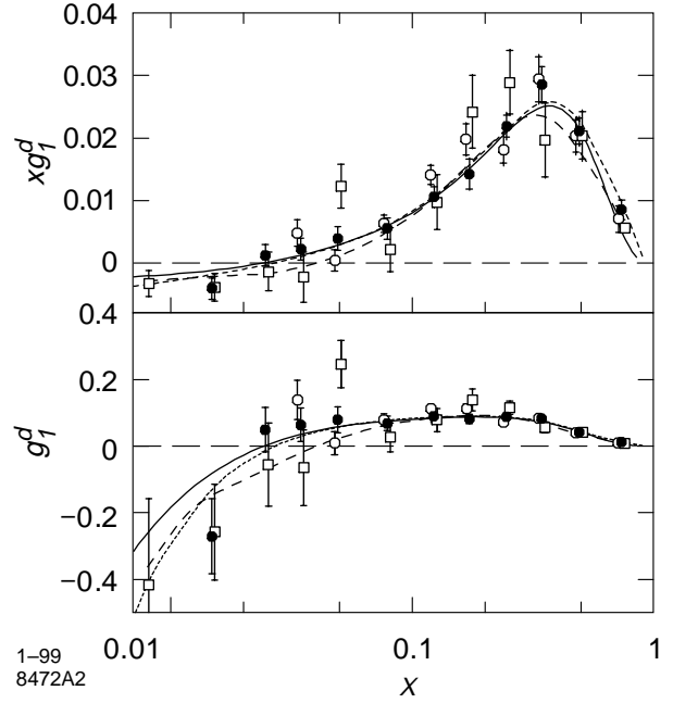
FIG. 2. Values of xg_1^d (a) and g_1^d (b) evolved to Q^2 of 5 (\text{GeV}/c)^2 using Eq. 4. The symbols and curves are as in Fig. 1.
