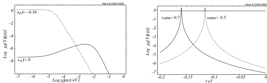
Figure 1. The baryon asymmetry Y_{B10} for vacuum oscillations of solar neutrinos ( m_{sun} = 10^{-5} eV) of as a function of the lightest neutrino mass m_1 (left) or the mixing angle s_{e3} (right). The plain curve on the left assumes CKM mixing, maximal atmospheric and solar mixing but vanishing s_{e3} while the dashed curve tunes s_{e3} to maximize M_1/M_2 and the asymmetry. The plot on the right shows the sensitivity of the baryon asymmetry on the mixing angle s_{e3} , most constrained by CHOOZ. For m_1 = m_{sun} = 10^{-5} eV, a sharp peak is obtained around s_{e3} \approx -0.22 s_{atm} .
