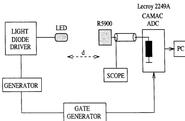
Figure 52 : Experimental set-up used for a first estimation of R5900 linearity .
