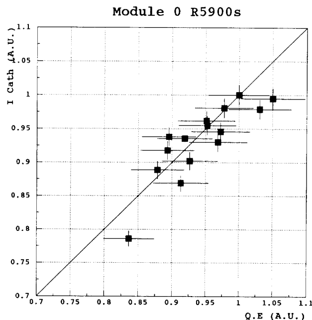
Figure 24 : Correlation between the estimated 480 nm quantum efficiency (x-axis), and the photocathode current measured at the "plateau" with the 480 nm interferential filter (y-axis). For the subset of tested PMTs, one of the PMT has been used as a reference (#5M18C3). We fix to 5% the systematic error on the relative estimated 480 nm quantum efficiency, and to 1.5% the systematic error on the relative photocathode current.
