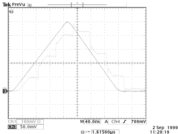
Figure 10: scope reproduction
