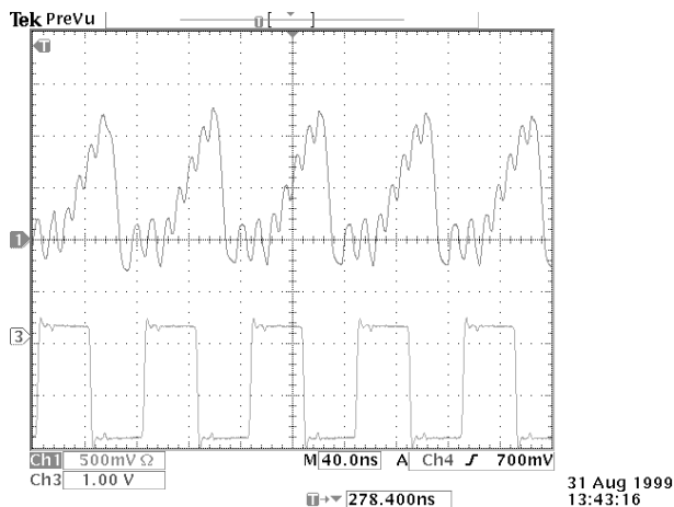
Figure 11: scope reproduction
