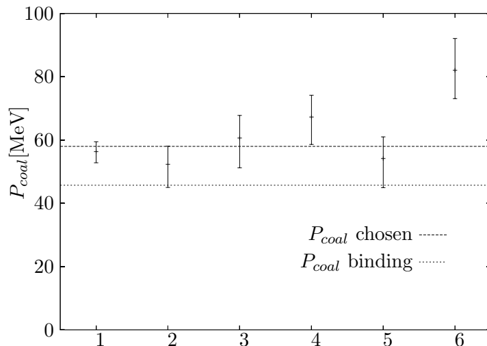
Figure 1: This figure displays various experimental constraints on the coalescence momentum P_{coal} , the only free parameter of the model discussed in the text. Points 1 and 2 are from Serpukhov with \sqrt{s}=11.5 GeV while all the other data have been collected at the ISR at \sqrt{s}=53 GeV. A coalescence momentum P_{coal} of order 60 MeV provides a reasonable fit of all the points but the last one. This value lies reassuringly close of the characteristic momentum derived from the binding energy of deuteron.
