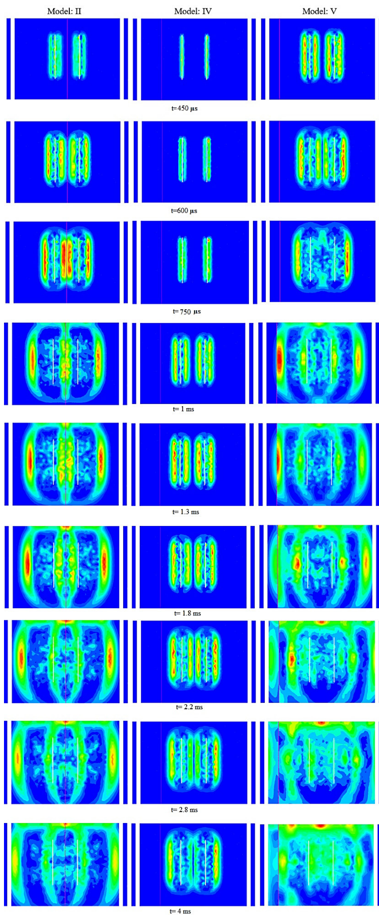
Figure 7: Blasting wave propagation in jointed rock of model #2, model #4, and model #5
