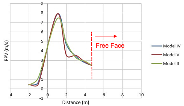
Figure 8: The peak particle velocity of models #2, #4, and #5
