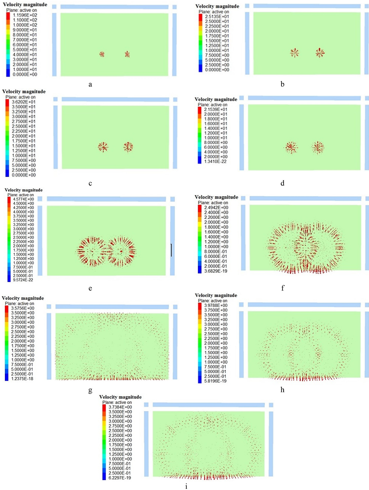
Figure 5: Plan of the blast wave propagation in intact rock (model #1) at a) 18µs b) 87µs c) 133µs d) 170µs e) 220µs f) 283µs g) 417 µsh) 550µs and i) 800µs
