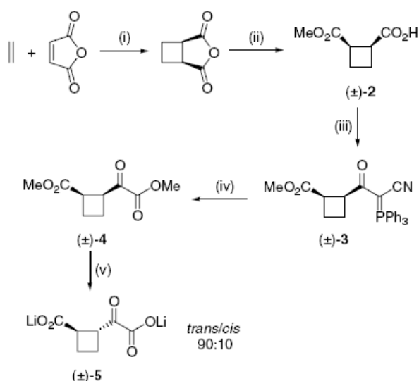
Scheme 1. Reagents and conditions: (i) acetophenone, \text{CH}_3\text{CN} , hv , pyrex, 5 h, 75%; (ii) MeOH, reflux, 16 h, 77%; (iii) (triphenylphosphoranylidene)acetonitrile, EDCI, DMAP, \text{CH}_2\text{Cl}_2 , rt, 4 h, 91%; (iv) \text{O}_3 , \text{CH}_2\text{Cl}_2/\text{MeOH} 3:1, -78^\circ\text{C} , 81%; (v) LiOH, MeOH, rt, 2 h then Dowex resin \text{H}^+ , 100%.
