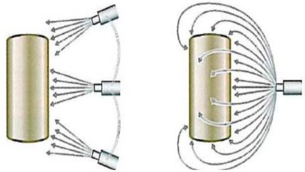
Figure 5: With ordinary spray guns (left) coating should be sprayed from different angles but with electrostatic spray guns (right) coating is adhered to a wide area from a single spray direction [22].
