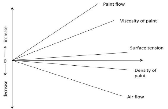
Figure 6: Influences on droplet size distribution during pneumatic atomization [8, 31].
