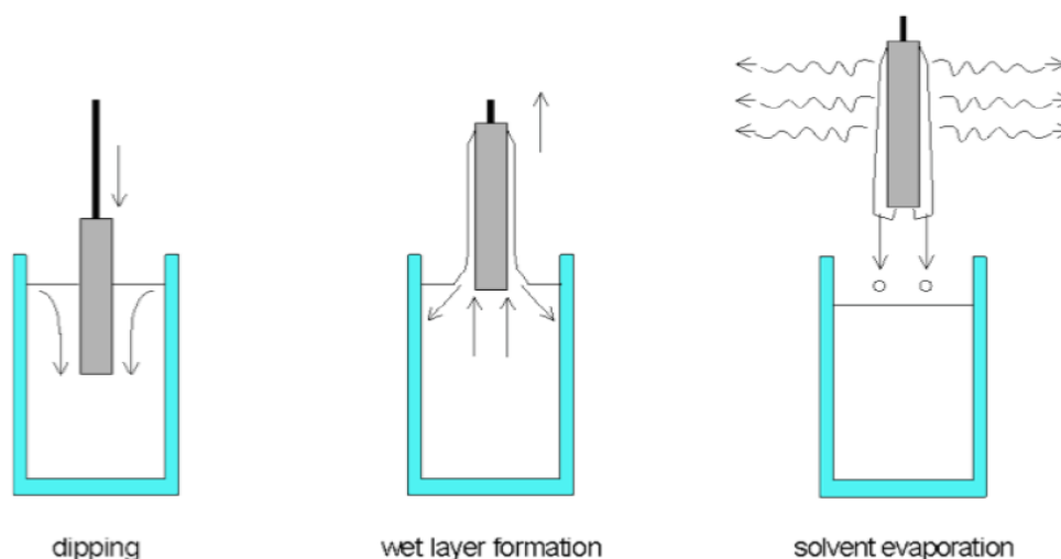
Figure 4: Sequential steps in a dip coating process [25].
