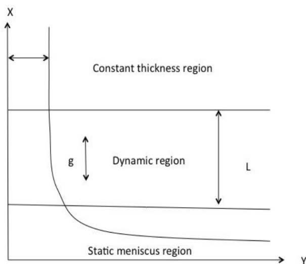
Figure 3: Schematic illustration of three separate regions in the thin film due to the vertical withdrawal of substrate from coating bath [21].
