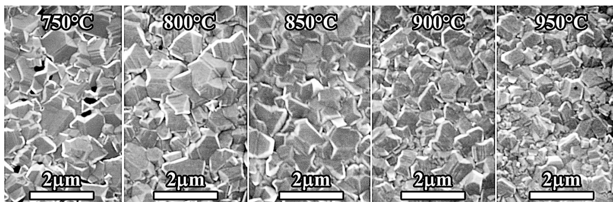
Figure 3: SEM images of Si-doped at \text{SiH}_4/\text{CH}_4 = 0.6\% diamond films grown at different substrate temperatures.
