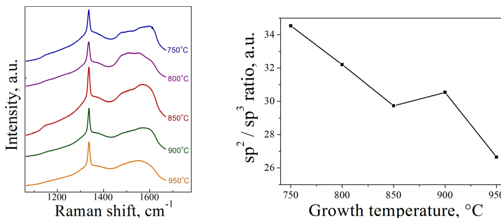
Figure 7: Raman spectra (left) and sp^2/sp^3 ratio for films prepared at different substrate temperatures at SiH_4/CH_4 = 0.6\% (right).
