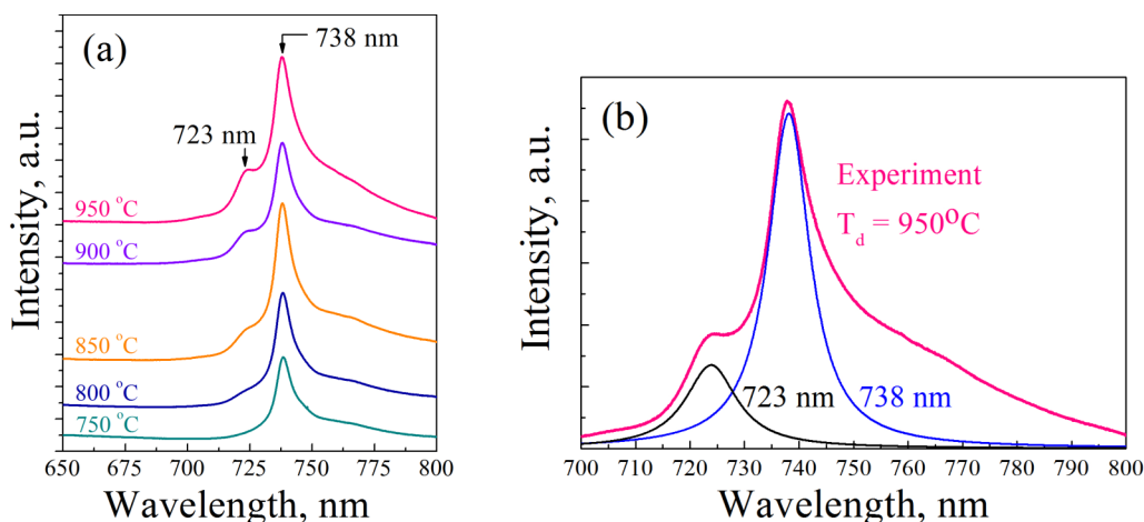
Figure 11: PL spectra for the films grown at different substrate temperatures at \text{SiH}_4/\text{CH}_4 = 0.6\% (a) and approximation of experimental line with two Lorentzians (b). Note the appearance of a side band at 723 nm for T_d > 800^\circ\text{C} .
