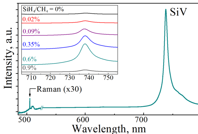
Figure 8: PL of diamond films grown at different SiH_4/CH_4 ratios, demonstrating the strong peak at 738\text{ nm} belonging to SiV defect. Note a decrease in PL for most doped sample ( SiH_4/CH_4 = 0.9\% ).
