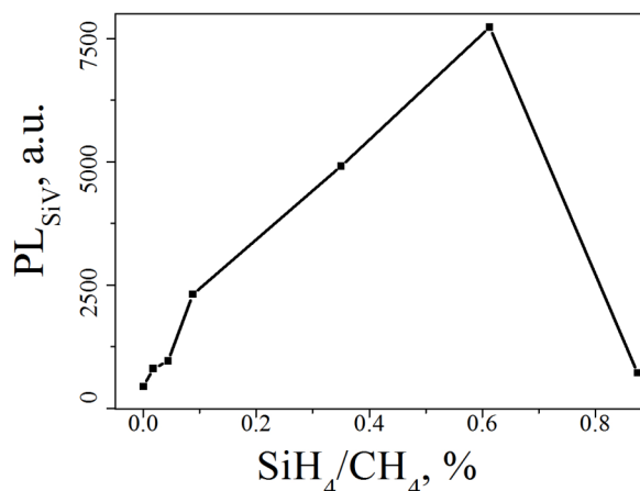
Figure 9: Dependence of integrated SiV PL intensity on SiH_4/CH_4 ratio used to deposit diamond films at 800^\circ\text{C} . The integrated SiV intensity is normalized to integrated diamond Raman peak intensity at 1336\text{ cm}^{-1} . The solid line is the guide for eyes.
