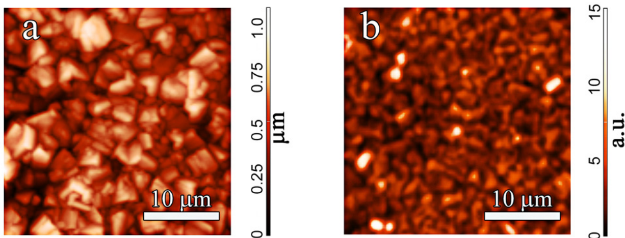
Figure 10: AFM image of a Si-doped microcrystalline diamond film grown at SiH_4/CH_4 = 0.6\% (a), and 738 nm PL map for the same region (b). The PL excitation was at 632 nm.
