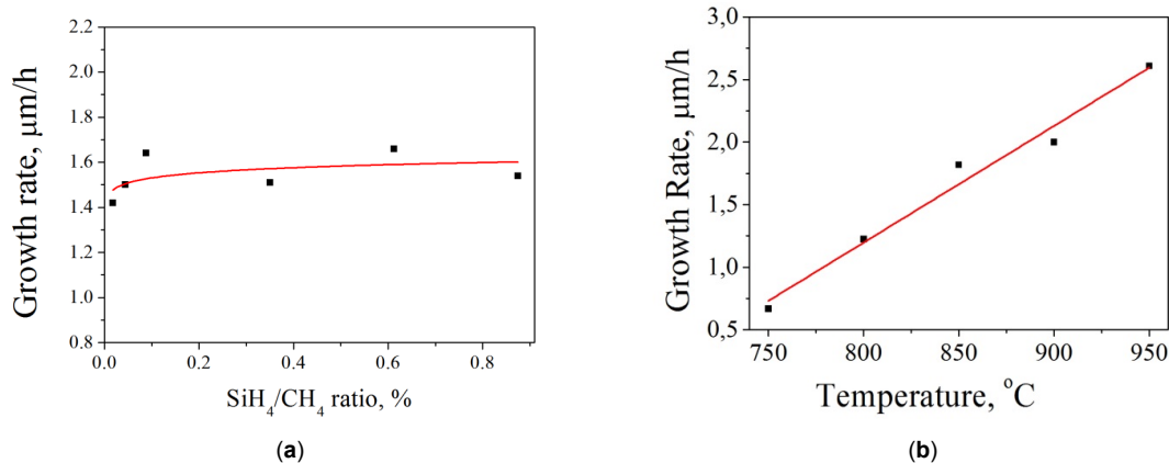
Figure 4: Dependencies of growth rate for the diamond films on \text{SiH}_4/\text{CH}_4 ratio at substrate temperature T_d=800^\circ\text{C} (a), and on substrate temperature at \text{SiH}_4/\text{CH}_4 = 0.6\% (b).
