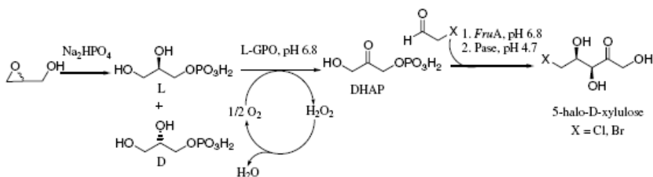
Scheme 1. Multienzyme system for one-pot 5-halo-D-xylulose synthesis.
