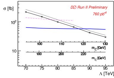
Figure 1. 95% C.L. limit on GMSB SUSY Snowmass Slope obtained in the analysis (thick blue line) and in the previous D\emptyset result (dot-dashed) purple-line. SUSY LO (NLO) cross-section is shown in black solid (dashed) line.
