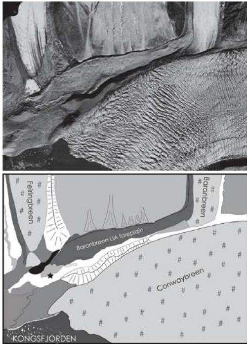
Figure 1. Aerial view of the Baronreen glacial foreplain
