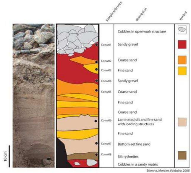
Figure 2 - Lithofacies of the Baronreen fan, Spitsbergen
