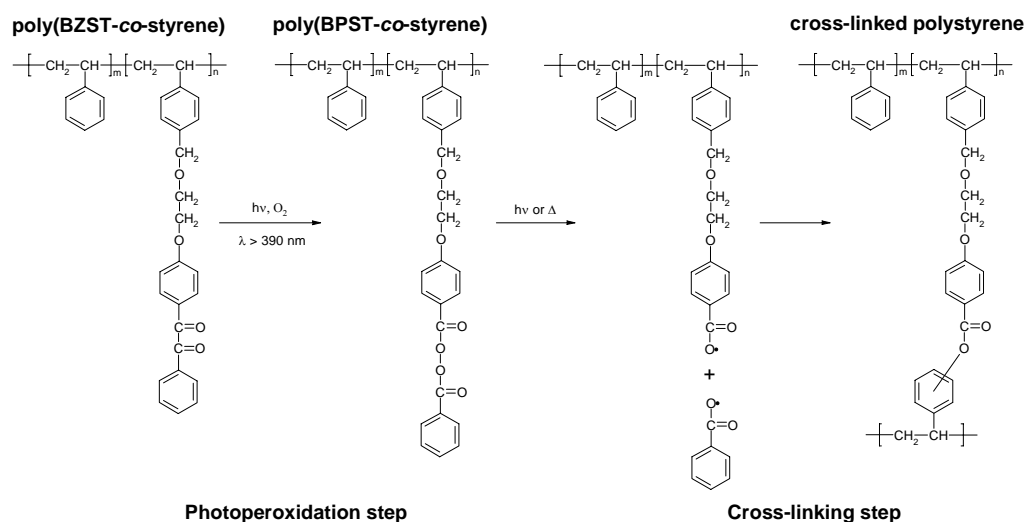
Scheme 1: Photo reactivity of poly(1-phenyl-2-(4-[2-(4-vinyl-benzyloxy)-ethoxy]-phenyl)-ethane-1,2-dione-co-styrene).
