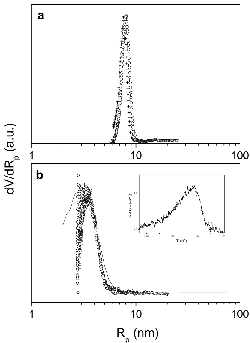
Figure 4: Pore size distributions derived from gas ( N_2 ) adsorption (lines) and from thermoporosimetry technique (symbols) for glassy beads with 7.5 nm of average pore radius (figure 4 a ) and for column chromatography silica gel (figure 4 b );. The inset figure shows the DSC thermogram of the solid-to-solid transition of CCl_4 within silica gel powder. (○) represents the PSD calculated from the solid-to-solid transition and (+) from the liquid-to-solid one, in Figure 4 b and because of the weak intensity of liquid-to-solid peak, only the solid-to-solid transition was used.
