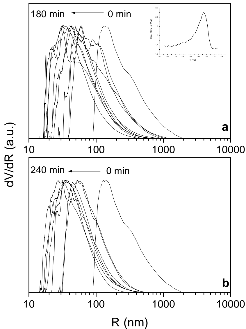
Figure 5: Mesh sizes distributions of the polymer networks of cross linked poly(BZST-co-styrene) samples. The films were at first irradiated in air at \lambda > 390 nm at 35^\circ\text{C} in order to transform the benzil pendant functions (BZ) into benzoyl peroxide groups (BP) and after then either thermally cross linked at 110^\circ\text{C} ( a ) or photo-cross linked by irradiation at \lambda > 300 nm at 35^\circ\text{C} ( b ). The inset figure shows an example of DSC thermogram of the liquid-to-solid transition of \text{CCl}_4 swelling a thermally cross linked copolymer sample.
