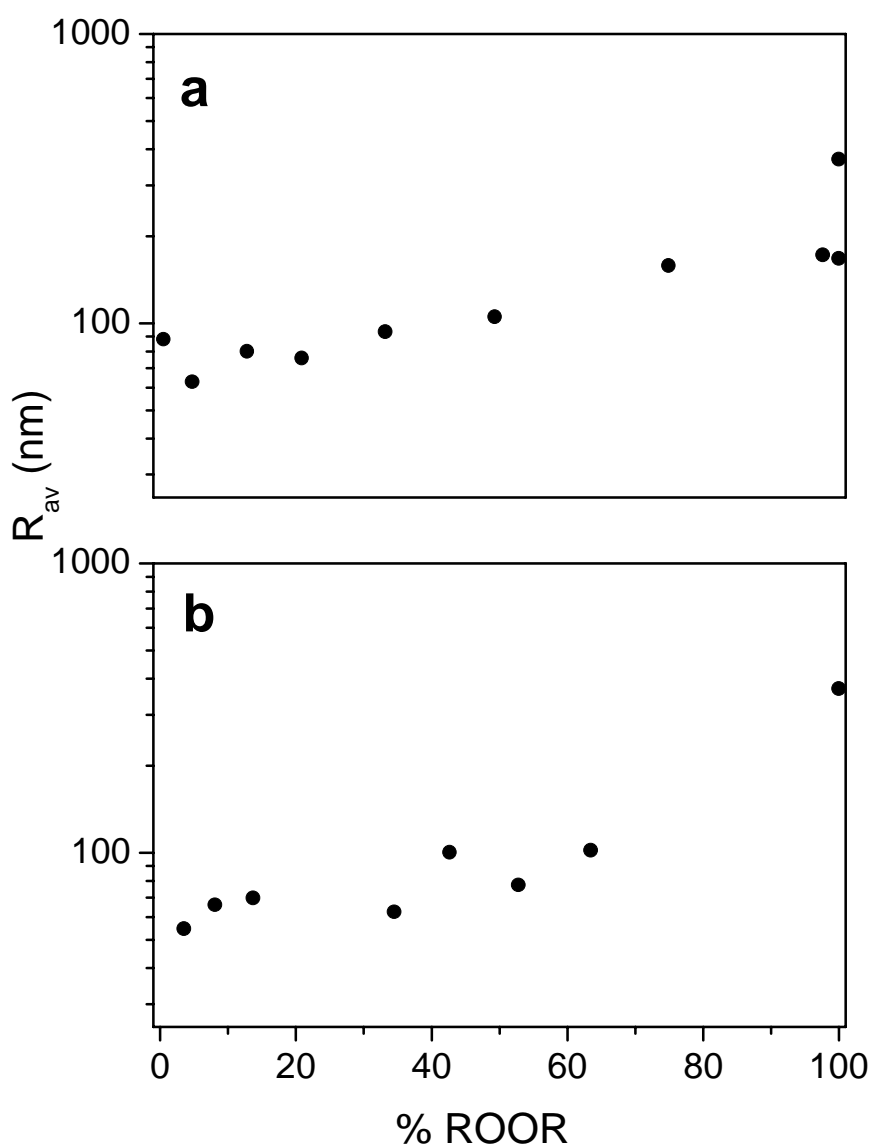
Figure 8: Correlation between the relative homolyzed benzoyl peroxide concentration (%ROOR) and the average mesh size ( R_{av} ) of the polymer network during irradiation at
