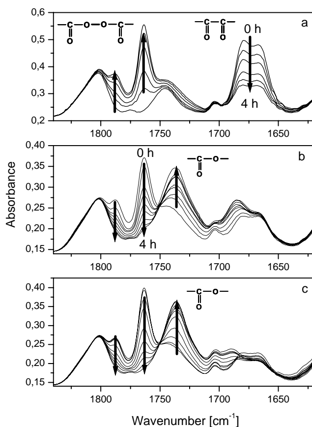
Figure 7: FTIR spectra of poly(VBZ-co-styrene) films. Peroxidation step: the films were irradiated at \lambda > 390\text{ nm} at 35^\circ\text{C} in air (a) . Cross linking step by thermal treatment: the peroxidized films were heated at 110^\circ\text{C} in aerated oven (b) . Photo-cross linking step :
