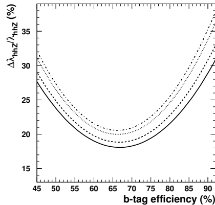
Figure 3: Expected resolution on the \lambda_{\text{hhh}} as a function of \epsilon_b . From down to up \frac{\Delta E}{\sqrt{E}}=0\% , 30%, 60% and 130%.
