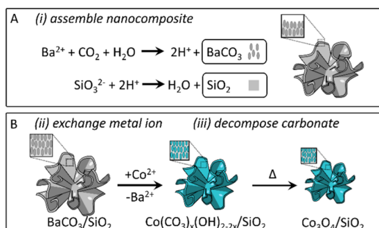
Figure 1. Preparation of catalytic nanocomposites. (A) Coprecipitation of nanocomposites containing BaCO 3 nanocrystals and amorphous SiO 2 . (B) Nanocrystals of the composites are converted by replacing the Ba 2+ with Co 2+ followed by decomposition to Co 3 O 4 , which serves as the precursor of the Fischer–Tropsch catalyst. 42
