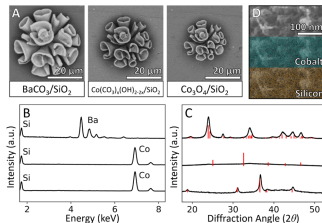
Figure 2. Shape-preserving conversion of BaCO 3 /SiO 2 to Co 3 O 4 /SiO 2 nanocomposites. (A) SEM images of self-assembled nanocomposites before exchange (left, BaCO 3 /SiO 2 ), after cation exchange (middle, Co(CO 3 ) x (OH) 2–2x /SiO 2 ), and after decomposition (right, Co 3 O 4 /SiO 2 ). (B) EDS analysis showing the presence of barium and silica in the initial BaCO 3 /SiO 2 nanocomposite (top), the replacement of Ba 2+ for Co 2+ after the cation exchange (middle), and the preservation of the metal-to-silicon ratio after decomposition (bottom). (C) XRD data of the initial BaCO 3 (top, orthorhombic), intermediate Co(CO 3 ) x (OH) 2–2x (middle, amorphous), and Co 3 O 4 (bottom, cubic). Reference lines in red show peaks measured in literature (COD 1000033, COD 1548825, and ICSD 27498 respectively, see Sections S1–S5 for details). (D) High-resolution SEM image of the Co 3 O 4 /SiO 2 nanocomposite surface (top), with corresponding EDS overlay showing the distribution of cobalt (cyan, middle) and silicon (brown, bottom).
