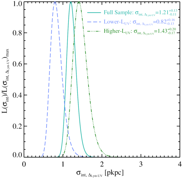
Figure B1. Likelihood distribution of the intrinsic projected one-dimensional spread of \Delta_{Ly\alpha-UV} for the full (solid teal), lower-luminosity (dashed light blue), and higher-luminosity (dot-dashed green) samples. The likelihood is calculated by the expression given in Equation B1. The median of the likelihood distribution for each sample along with their corresponding effective 1\sigma confidence interval is shown in the top right. As in other analyses, offsets are found to be significantly higher for galaxies that are brighter in the UV.
