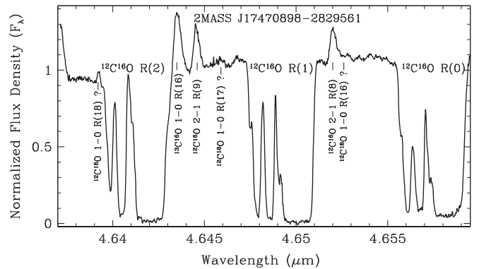
Figure 5. High-resolution spectrum covering the lowest three lines of the R branch of the fundamental band of ^{12}\text{C}^{16}\text{O} , observed by Phoenix at Gemini South.
