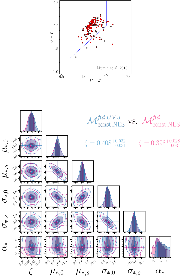
Figure 1. Top panel: UVJ colour-colour diagram for the LEGA-C sample of 178 ETGs (red dots). The broken line separates quiescent (upper-left region) and star-forming galaxies (lower-right region) as in Muzzin et al. (2013). Bottom panel: posterior probability distributions of the hyper-parameters for the M_*\text{-}\sigma_e models \mathcal{M}_{\text{const,NES}}^{\text{fid}} (purple contours) and \mathcal{M}_{\text{const,NES}}^{\text{fid,UVJ}} (blue contours). In the 1D distributions (top panel of each column) the vertical solid lines and colours delimit the 68, 95 and 99.7-th quantile based posterior credible interval. In the 2D distributions (all the other panels) the contours enclose the 68, 95 and 99.7 percent posterior credible regions. The lines indicate the median values of the hyper-parameters.
