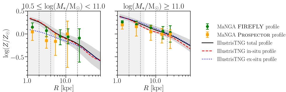
Figure 2. Mass-weighted metallicity radial profiles of massive ETGs with lower (left panel) and higher (right panel) stellar mass. The circles and squares represent the median estimates for MaNGA galaxies from FIREFLY and PROSPECTOR codes, respectively. The curves represent the median estimates for IllustrisTNG galaxies. The dashed and dotted curves represent the in-situ and the ex-situ stellar components, respectively, while the solid curve represents the total stellar components. The shaded area and the error bars indicate 1\sigma scatter.
