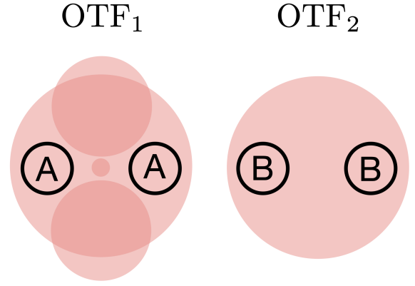
Fig. 5. Regions in the OTF_1 and OTF_2 that are not contaminated by the sidebands or the RH. Therefore, regions A and B are suitable to measure p .
