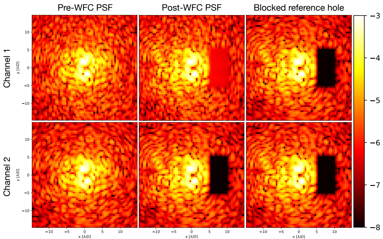
Fig. 12. WFC example with the PESCC without noise sources present. The subfigures in the two rows show the PSFs of the two channels. The columns show, respectively, the PSFs before WFC, the PSFs after twenty iterations of the WFC, and the PSFs after the WFC with the RH blocked. The colorbar shows the intensity in logarithmic scale and is equal for all subfigures.
