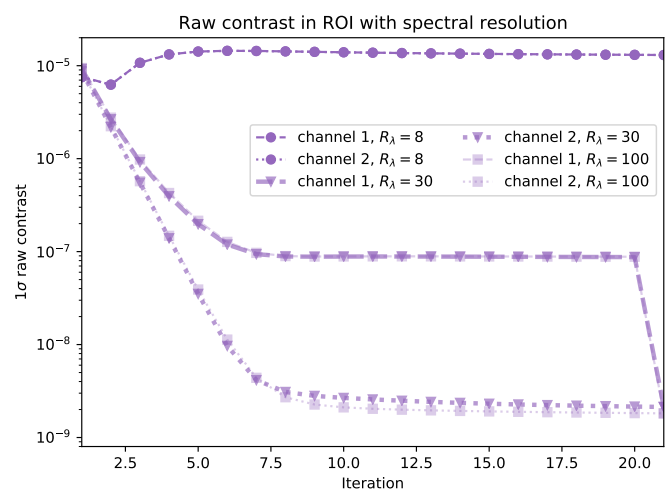
Fig. 18. Raw contrast as function of iterations for the system with broadband effects. The response matrix is acquired with the broadband effects included. At iteration 21, the RH is blocked to compare the raw contrast in the two channels.
