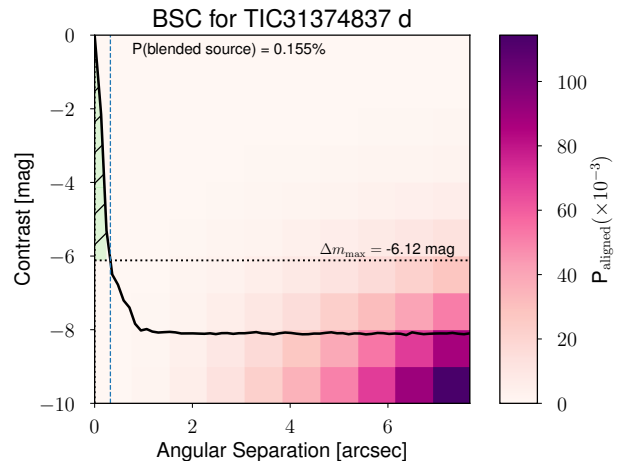
Figure 2. Contrast curve of TOI-431 from the Keck/NIRC2 instrument for the Ks filter (solid black line). The colour ( P_{aligned} ) on each angular separation and contrast bin represents the probability of a chance-aligned source with these properties at the location of the target, based on TRILEGAL model (see Sect. 2.3.5 within the main text). The maximum contrast of a blended binary capable of mimicking the planet transit depth is shown as a dotted horizontal line. The hatched green region between the contrast curve and the maximum contrast of a blended binary ( \Delta m_{max} line) represents the non-explored regime by the high-spatial resolution image. P(\text{blended source}) is the Blended Source Confidence (BSC), and this corresponds to the integration of P_{aligned} over the shaded region.
