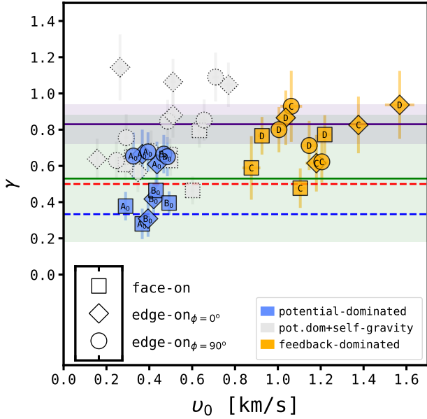
Figure 5. Structure function parameters ( \nu_0 , \gamma ) of cloud complexes extracted from different physical scenarios (marker colour) and orientations (marker style) using the Mixed method. Solid lines (and their errors as shades) are reference literature values whose legends can be found in Table 2. Markers in gray are potential-dominated self-gravitating complexes studied separately in Sec. 6.3 as a function of time.
