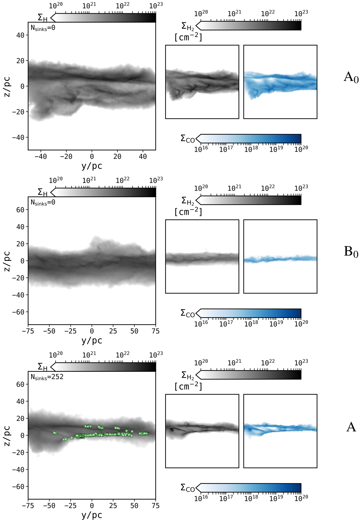
Figure A3. Edge-on \phi=90^\circ projections of H , H_2 and ^{12}CO column densities ( \Sigma ) from cloud complexes (labeled on the right) extracted 2 Myr after injecting tracer particles in the simulations. If any, sink particles are overlaid on H maps as star markers.
