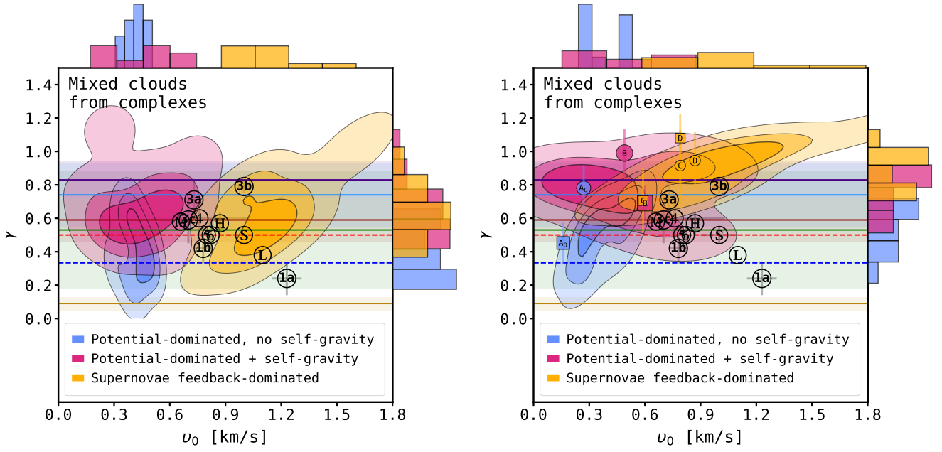
Figure A6. Same as left panel of Fig. 8 but using LTE (left) and LVG (right) level populations for the radiative transfer of ^{12}\text{CO} from our cloud complexes. Coloured markers in the right panel are the ^{13}\text{CO} parameters presented in Table 4.
