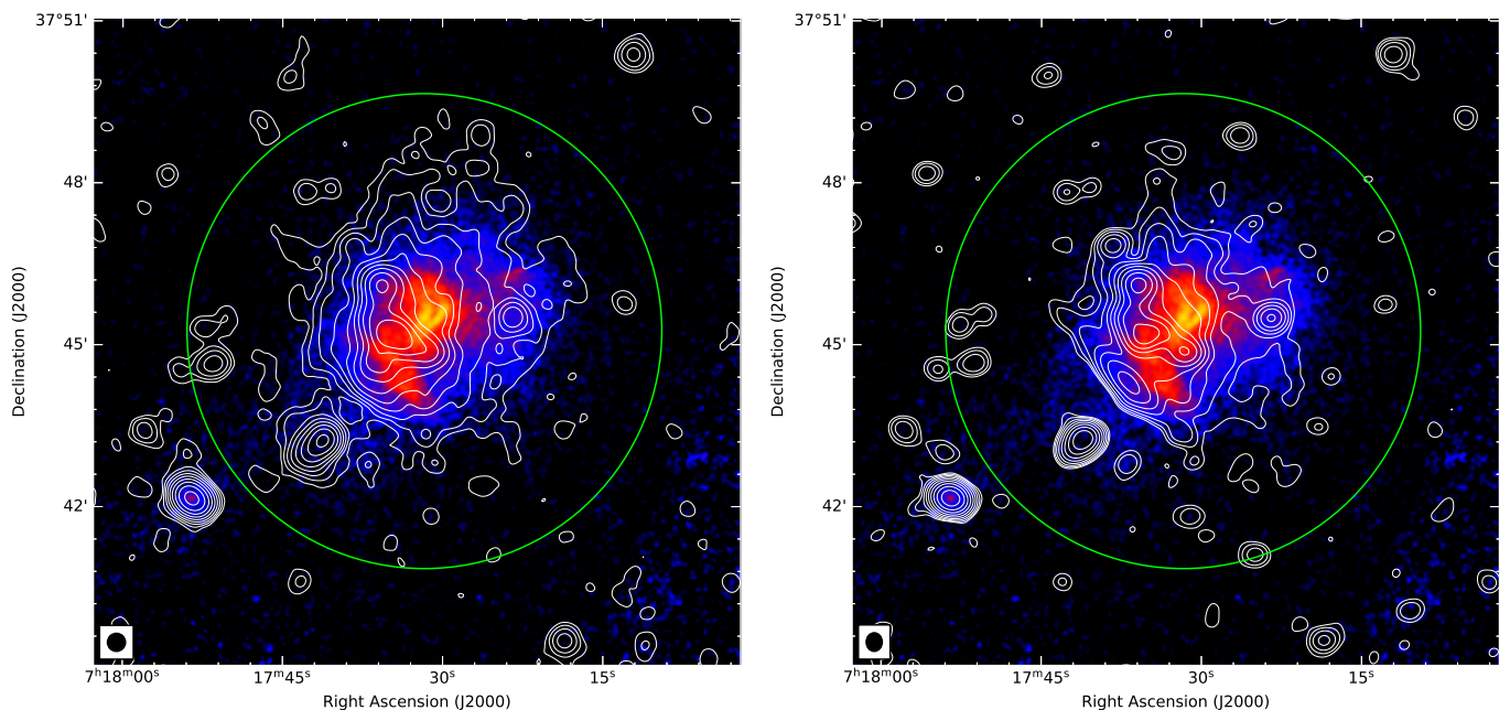
Fig. 10. Low resolution ( 20'' ) LOFAR ( left ) and VLA L-band ( right ) radio contours, superimposed on the Chandra X-ray ( 0.5 – 2 keV) image, smoothed to a FWHM of 3'' . Contour levels are drawn at [1, 2, 4, 8, \dots] \times 4\sigma_{\text{rms}} , where \sigma_{\text{rms}} at 144 MHz and 1.5 GHz are 130 \mu\text{Jy beam}^{-1} and 14 \mu\text{Jy beam}^{-1} respectively. The radio halo shows a strikingly similar morphology to the ICM distribution (traced by the X-ray emission), confirming the connection between the hot gas and relativistic plasma. The emission from the radio halo at 144 MHz, further extends over the whole region of detected X-ray emission. The green circle shows R_{500} for the cluster.
