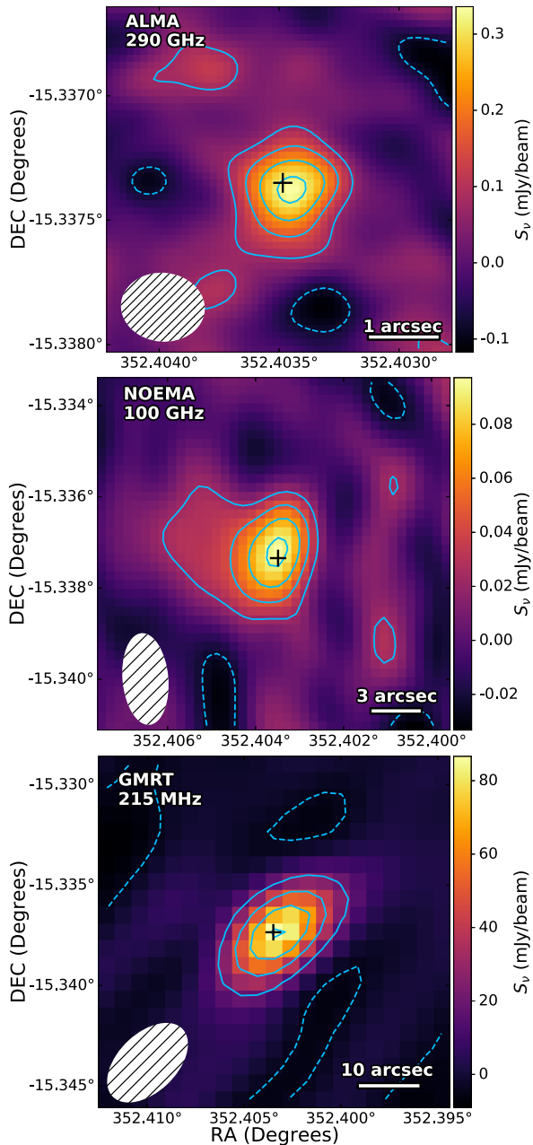
Figure 3. Top: ALMA 290 GHz continuum emission map of P352–15, with an RMS \sigma = 0.04 \text{ mJy beam}^{-1} . The beam size is 1''.3 \times 1''.0 and the quasar is unresolved. Middle: NOEMA 100 GHz continuum emission map with \sigma = 0.01 \text{ mJy beam}^{-1} . The beam size is 7''.3 \times 3''.7 and the quasar is unresolved. Bottom: GMRT 215 MHz emission map with a beam size of 18'' \times 11'' and \sigma = 4 \text{ mJy beam}^{-1} . The quasar appears unresolved. The contour levels for ALMA and NOEMA maps are shown at (-2, 2, 4, 6, 8)\sigma and both have S/N > 8 . The GMRT continuum has contours shown at (-1, 5, 10, 15, 20)\sigma and has S/N > 20 . For all maps, the dashed and solid contours represent the negative and positive \sigma , respectively. The cross in all panels is centered at the optical position of P352–15 from Momjian et al. (2018).
