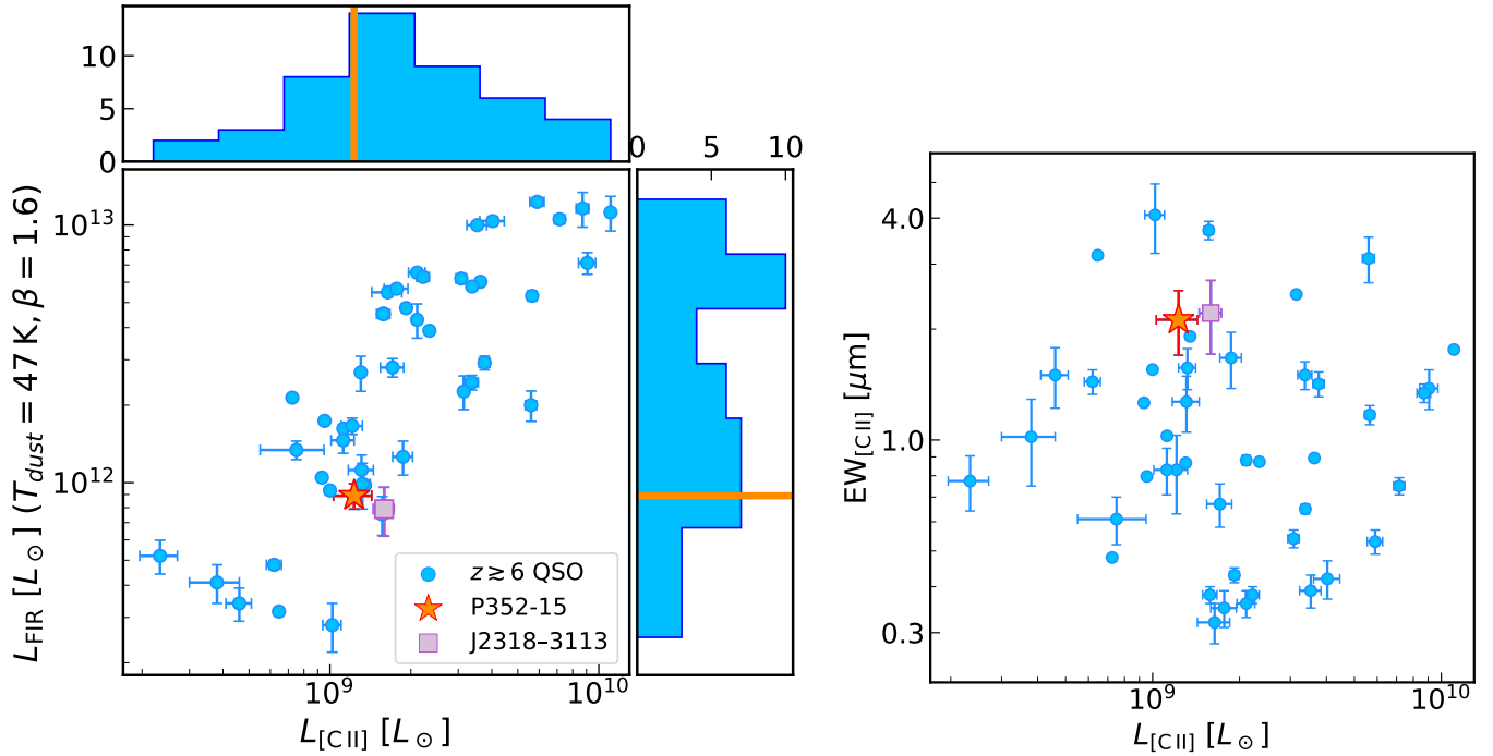
Figure 5. Left: Relationship between the FIR luminosity (assuming is dominated by cold dust with T_{Dust} = 47 K and \beta = 1.6 ), and the [C II] luminosity reported in 45 z \gtrsim 6 quasars from Decarli et al. (2018); Izumi et al. (2018); Eilers et al. (2020, 2021); Venemans et al. (2020). The derived properties of P352–15 are within typical values for L_{\text{FIR}} and L_{\text{[C II]}} in context with the literature. Right: Comparison between the [C II] equivalent width and the [C II] luminosity using the same sample of z \gtrsim 6 quasars. P352–15’s \text{EW}_{\text{[C II]}} value is at the high end of the distribution found in the literature. The two panels also highlight J2318–3113, the only other radio-loud quasar in the z \gtrsim 6 sample with available information for comparison. Both radio-loud quasars have very similar [C II] and FIR properties.
