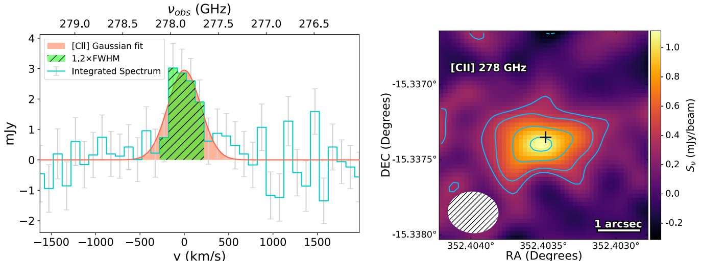
Figure 1. Left: ALMA continuum-subtracted [C II] emission of P352–15. We use a 1''.7 aperture radius to extract the emission line spectra presented here in blue. The error bars represent the RMS within the aperture at each channel. The spectral range used for the Gaussian fit of [C II] is shaded in orange and corresponds to a velocity-integrated value of 1.37 \pm 0.22 \text{ Jy km s}^{-1} . The [C II] fit at peak has a flux density of 2.95 \pm 0.48 \text{ mJy} . The hatched area in green corresponds to \approx 1.2 \times \text{FWHM} of the Gaussian fit and is used to create the [C II] map shown in the right panel. Right: 2D map of [C II] built with the data from the channels shown in the left panel in green. The emission is marginally resolved and the contour levels are shown at (-2, 2, 3, 5, 7)\sigma with \sigma = 0.15 \text{ mJy beam}^{-1} where the Beam is 1''.3 \times 1''.0 . The [C II] line is detected at \text{S/N} > 7.5 . The cross is centered at the optical position of P352–15 from Momjian et al. (2018).
