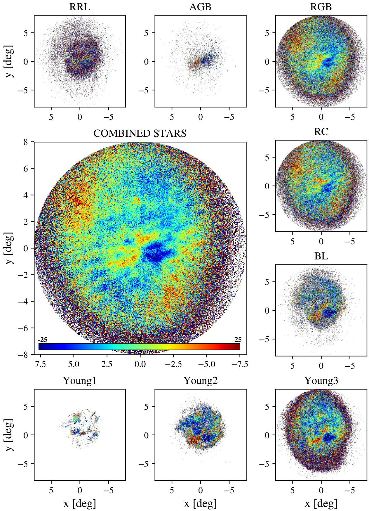
Fig. B.2: Radial velocity maps v_R of the LMC for the combined sample (main panel) and the various evolutionary phases. The linear velocity scale shown by the colour bar in the main panel is the same in all subpanels and has been chosen to highlight velocity patterns better.
