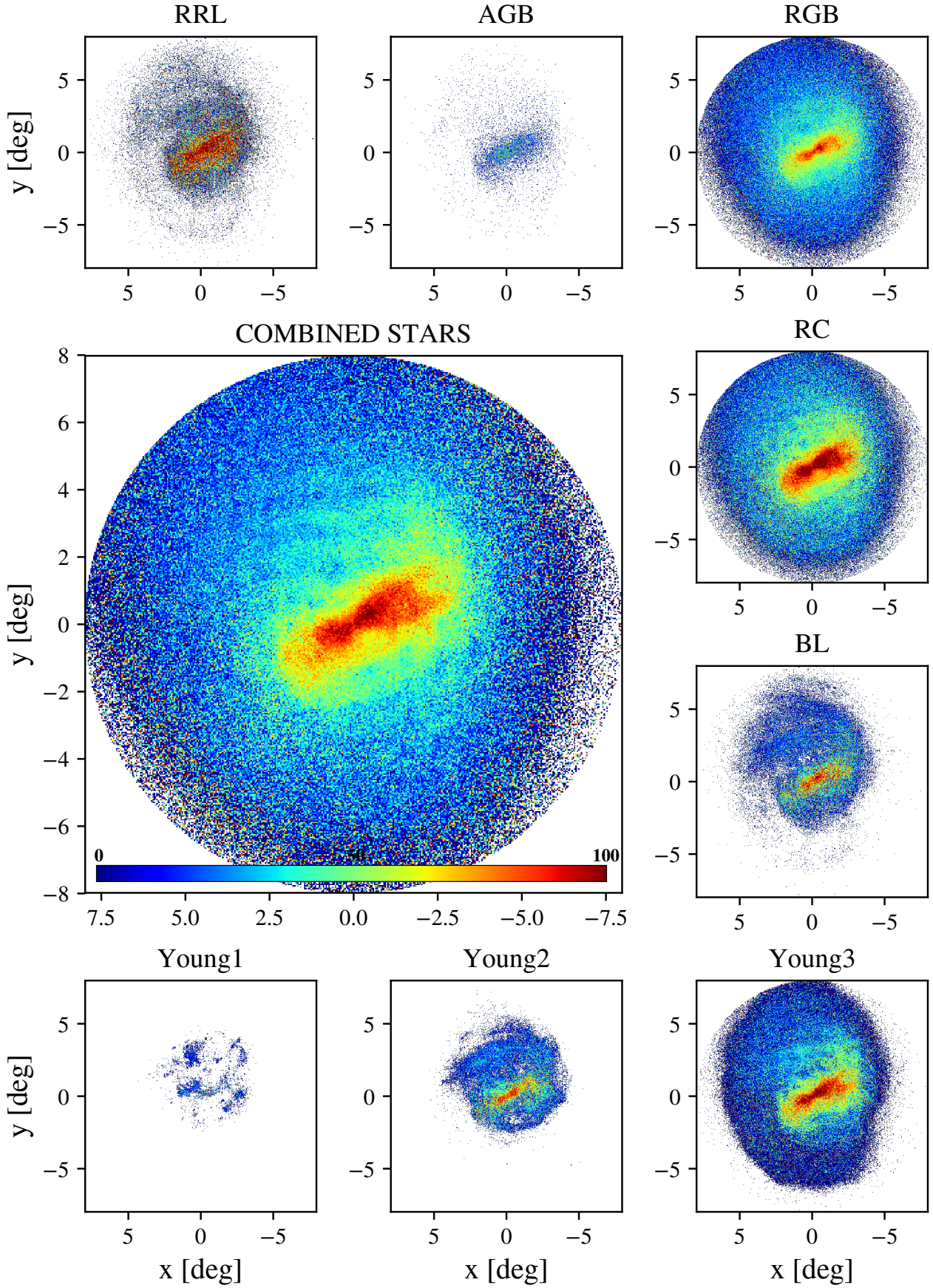
Fig. B.3: Azimuthal velocity dispersion maps \sigma_\phi of the LMC for the combined sample (main panel) and the various evolutionary phases. The linear velocity scale shown by the colour bar in the main panel is the same in all subpanels and has been chosen to highlight velocity patterns better.
