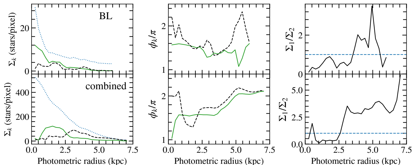
Fig. 19: Results of the Fourier transform of stellar density maps of the LMC for the BL and the combined samples (upper and bottom panels, respectively). The left and middle panels show the amplitude and phases of the first- and second-order asymmetries (dashed black and solid green lines, respectively). The axisymmetric density is shown as a dotted blue line. The right panel shows the k = 1 perturbation over the bisymmetry strength ratio. The galactocentric radius is given here in the photometric frame, with \Omega_{\text{phot}} = 10^\circ as the reference photometric position angle.
