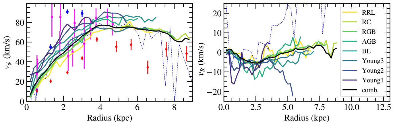
Fig. 14: Stellar velocity curves of the LMC. The left and right panels show the rotation curves and radial motions, respectively. Coloured lines are for the eight evolutionary phases and the combined sample, as given by the legend. In the left panel, blue circles, red diamonds and magenta squares are the rotation velocities for the samples of younger and older stars from line-of-sight spectroscopic and HST astrometric measurements published in van der Marel & Kallivayalil (2014). The dashed blue lines are the tangential and radial velocity profiles derived by Wan et al. (2020) from Gaia DR2 astrometry.
