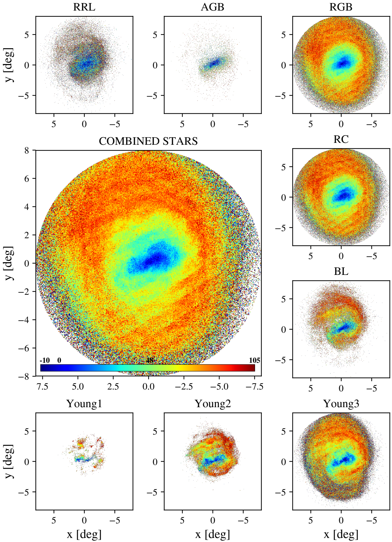
Fig. B.1: Azimuthal velocity maps v_\phi of the LMC for the combined sample (main panel) and the various evolutionary phases. The linear velocity scale shown by the colour bar in the main panel is the same in all subpanels and has been chosen to highlight velocity patterns better.
