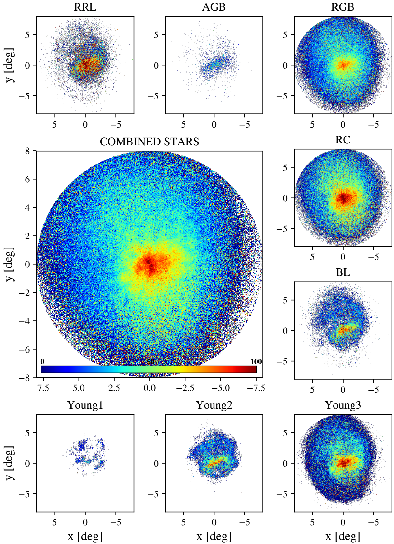
Fig. B.4: Radial velocity dispersion maps \sigma_R of the LMC for the combined sample (main panel) and the various evolutionary phases. The linear velocity scale shown by the colour bar in the main panel is the same in all subpanels and has been chosen to highlight velocity patterns better.
