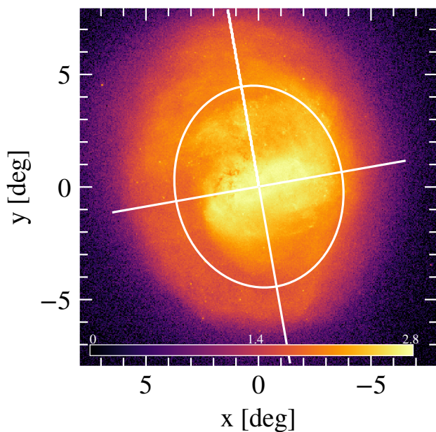
Fig. 20: Stellar density map of the combined sample of the LMC. The lopsided eastern spiral arm is located beyond R_{\text{phot}} = 3.8 kpc (shown as an ellipse). The perpendicular axes show the orientation of the photometric major and minor axes (Sect. 7.2). The density scale shown by the colour bar is logarithmic; the values indicate the star count in pixels.
