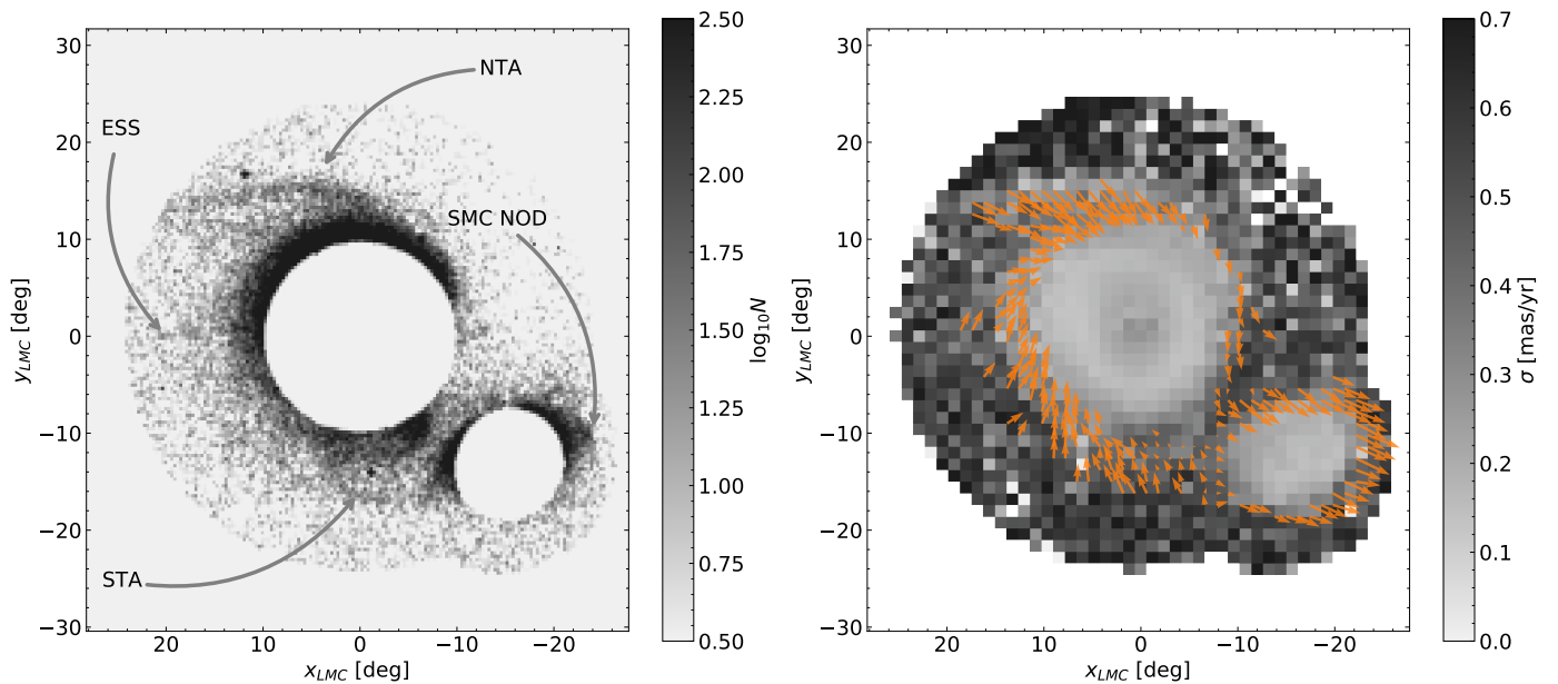
Fig. 17: Number count map for the LMCout sample (left): the names of the most notable substructures are given and, for a better visualisation, the inner parts of the LMC and SMC were omitted. Total velocity dispersion map (right): the velocity vector field is shown as orange arrows.
