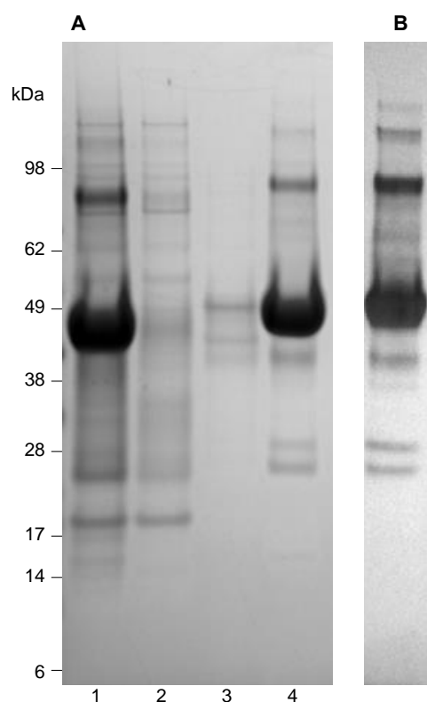
Figure 1. (A) Coomassie-stained SDS-PAGE gel showing the purification procedure of USUV E protein from E. coli , starting with isolated inclusion bodies. Lane 1, inclusion bodies solubilized in 20 mM Tris, 8.0 M urea, pH 8.0, prior to application on the Ni-IMAC column; lane 2, Flow-through; lane 3, wash with 20 mM Tris, 8.0 M urea pH 8.0, 10 mM imidazole; lane 4, elution with 20 mM Tris, 8.0 M urea pH 8.0, 100 mM imidazole. (B) Western blot analysis of the purified USUV E protein (as in lane 4 of panel A), developed using mouse anti-HIS as the primary antibody.
