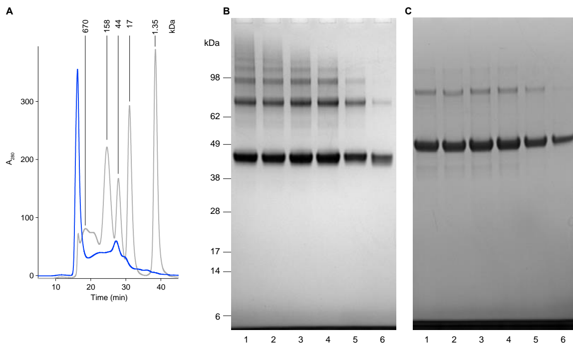
Figure 2. (A) Size-exclusion chromatography of USUV E protein fraction after a refolding procedure using rapid dilution (blue line), compared to a mixture of protein markers (grey line) with their molecular mass indicated. (B) SDS-PAGE analysis (non-reduced) of collected 1 mL fractions of the SE-chromatography. Lanes 1; fraction 16–18 min; lanes 2, 18–20 min; lanes 3, 20–22 min, lanes 4, 22–24 min, lanes 5, 24–26 min, and lanes 6, 26–28 min. (C) SDS-PAGE analysis (non-reduced) of collected 1 mL fractions of the SE-chromatography. Lanes are identical as described for Panel B.
