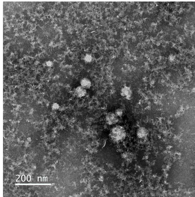
Figure 3. Electron microscopic analysis of purified USUV E protein. Purified USUV E antigen was negatively-stained with PTA and examined under EM. The scale bar indicates a size of 200 nm.
