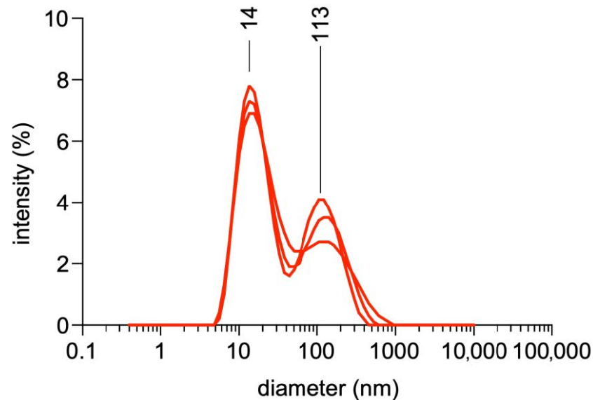
Figure 4. Dynamic Light Scattering analysis of the USUV E protein fraction showing the intensity-weighted particle distribution profile.
