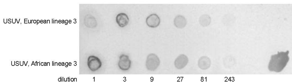
Figure 6. Dot blot of heat-inactivated supernatants of Vero cell-grown USUV strains, stained with pooled rabbit serum of USUV E protein-immunized rabbits. Upper row: USUV, European lineage 3 isolate; lower row, supernatants of USUV, African lineage 3. Supernatants were concentrated and spotted in a 1:3 dilution series. The spot to the right is a positive control, containing the immunogen ( E.coli -produced USUV E protein).
