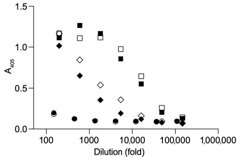
Figure 5. ELISA of two rabbit sera obtained after immunization, including 2 control sera after immunization with a control protein purified using a highly similar procedure. Squares represent day 28 (final bleed) sera from USUV E protein immunized animals, open symbol is serum 710, closed is serum 711. Diamonds represents 2 sera of control protein immunized animals, for which the protein was purified in a highly similar fashion. Circles represent pre-bleed sera from rabbits 710 (open) and 711 (closed). Starting dilution was 1:150.
