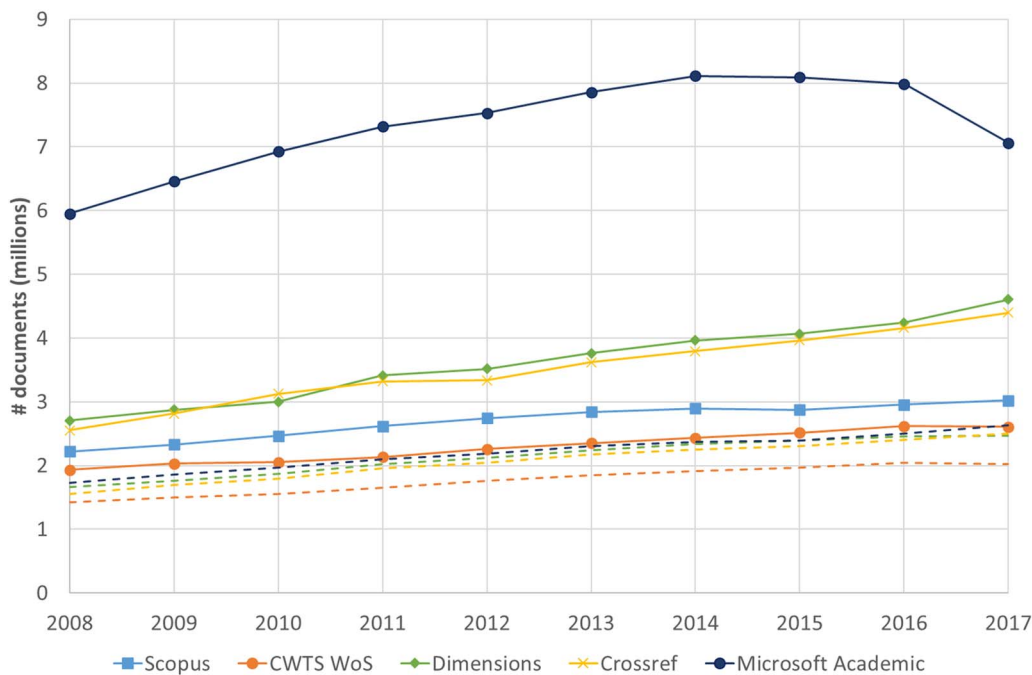
Figure 2. Breakdown by publication year for all documents in each data source (solid line) and for the overlap with Scopus (dashed line).
