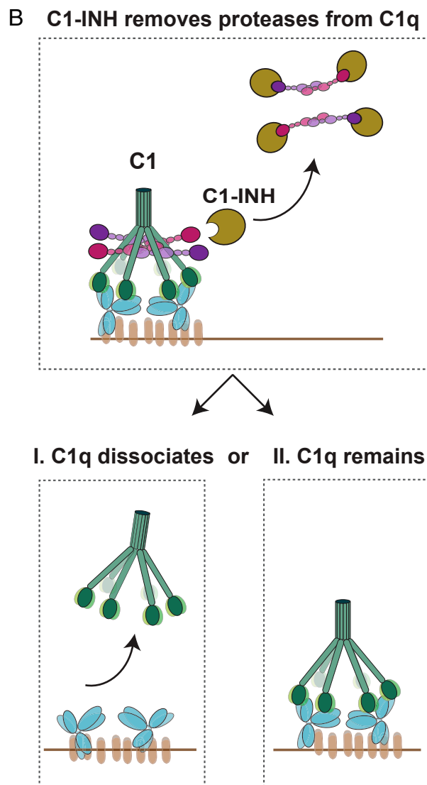
Fig. 4. Removal of C1 r2s2 proteases from surface-bound C1–IgG complexes can result in C1q dissociation. (A) Detection of C1q on IgG-coated DNP beads that were first labeled with purified C1 and subsequently incubated with 10 mM EDTA or 200 nM C1-INH to remove C1r and C1s proteases. The data represent geometric mean \pm SD of three independent experiments. Unpaired Student's t test (buffer versus EDTA; buffer versus C1-INH); * P < 0.05, all other conditions not significant. (B) Schematic cartoon of our hypothesis that C1 r2s2 dissociation by C1-INH can result in C1q dislodgement depending on the stability of the C1q–IgG complex. Our data suggest that removal of the C1r and C1s proteases from surface-bound C1 by C1-INH can result in two situations: 1)
