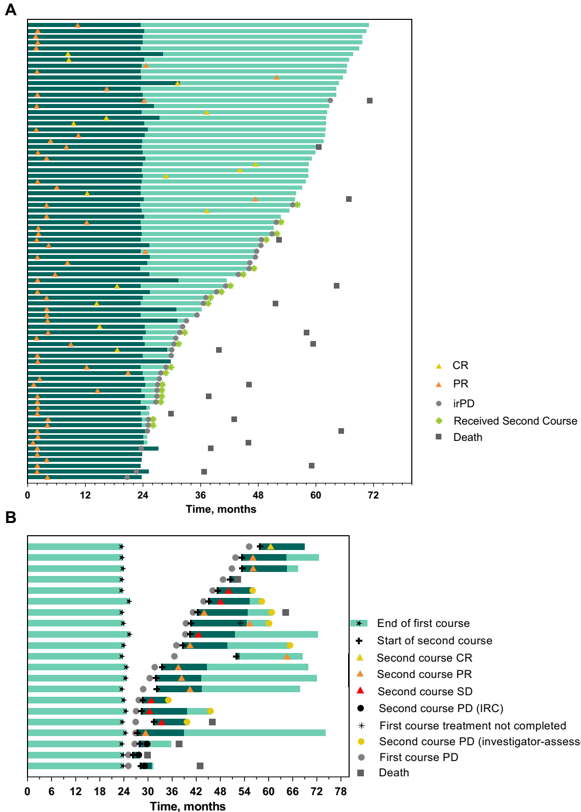
Figure 3. (A) Outcomes in patients who completed 35 cycles of pembrolizumab. Bar lengths indicate duration of treatment (dark green) and months of follow-up (light green). Follow-up was defined as date of the last known nonprogression scan or date of last investigator assessment the patient was alive. Response evaluation is per RECIST version 1.1 by independent central assessment. (B) Outcomes in patients who started second-course pembrolizumab. Bar lengths indicate duration of second-course treatment (dark green) and months of second-course follow-up (light green bar after dark green bar). Follow-up was defined as the last known nonprogression scan or date of last investigator assessment the patient was alive. Response
