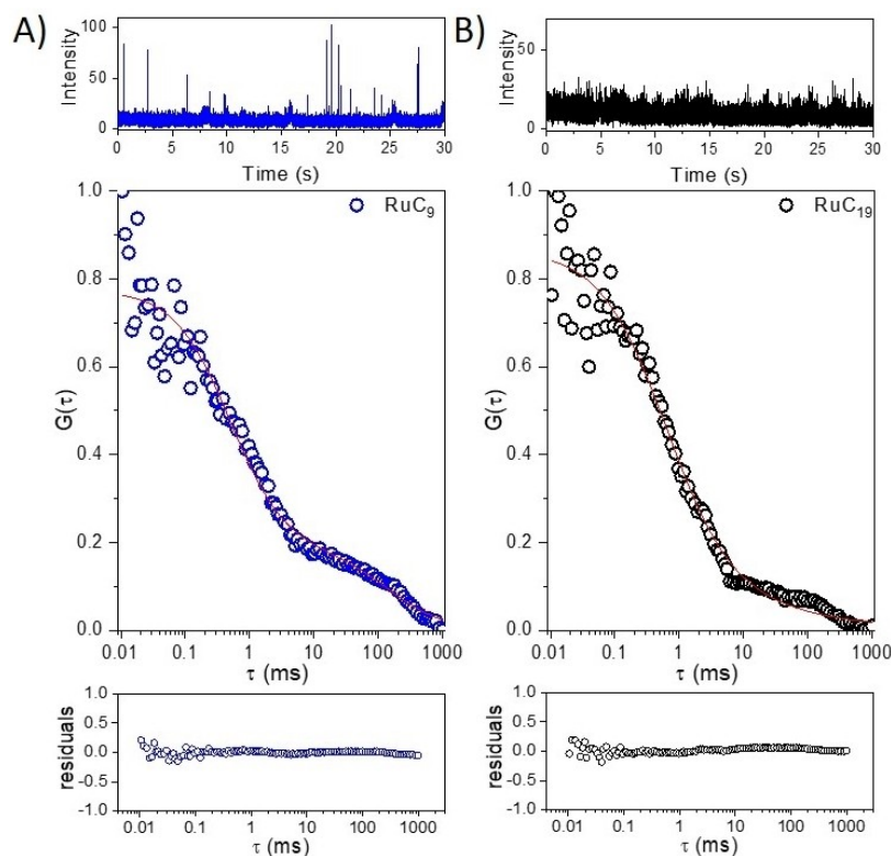
Figure 6. Representative intensity-time trace (top) and ACF (bottom) data measured over a single microcavity of MSLBs comprised of DPPC:NaDSPE-PEG2K: \text{RuC}_n in a ratio of 100:1:10^{-4} for (A) \text{RuC}_9 , and (B) \text{RuC}_{19} . The fit ACF to the two-component model is shown as the red line and bottom shows the residuals, that indicate the quality of the fit to the two-dimensional model of diffusion. Experimental conditions: [DPPC] = 1.36 mM, [NaDSPE-PEG2K] = 13.6 \mu\text{M} , and [ \text{RuC}_n ] = 40 nM in phosphate buffer saline (pH = 7.7). Bulk concentration [ \text{RuC}_n ] indicates theoretical concentration (before extrusion).
