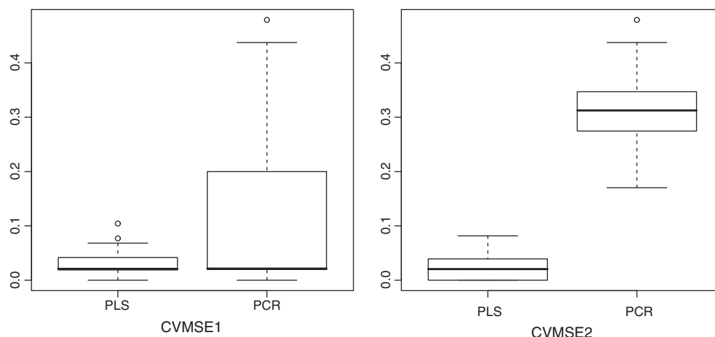
Fig. 17. Spectrometric data. Box plots for the distribution of the misclassification rate with FPLS and FPCR approaches and both model selection criteria on 150 test samples.
