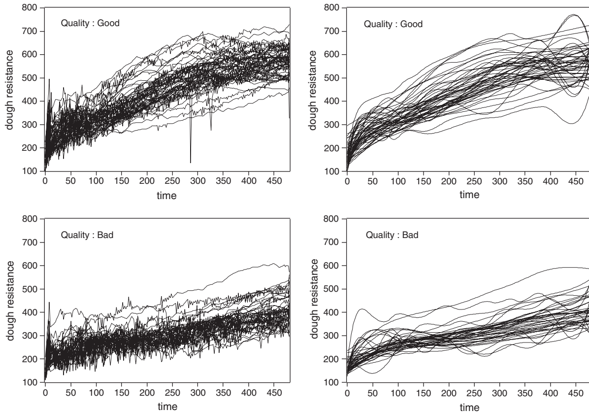
Fig. 14. Kneading data: 90 flours observed for 480 s. Left: observed data. Right: smoothed data using cubic B-splines.
