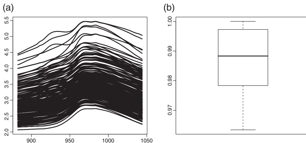
Fig. 16. Spectrometric data. (a) Sample of N=215 pieces of fine chopped meat. (b) Box and Whisker plot of correlation between columns of A\Phi matrix in spectrometric data.
