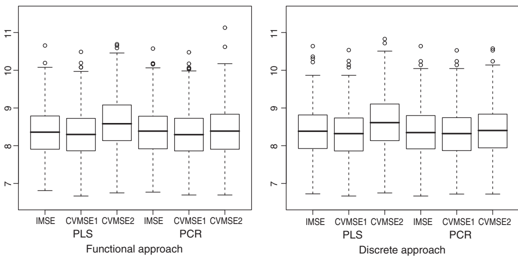
Fig. 11. Case II (CVMSE). Box plots for the distribution of CVMSE for the functional and discrete PLS and PCR models selected with the three considered criteria (IMSE, CVMSE1 and CVMSE2).
