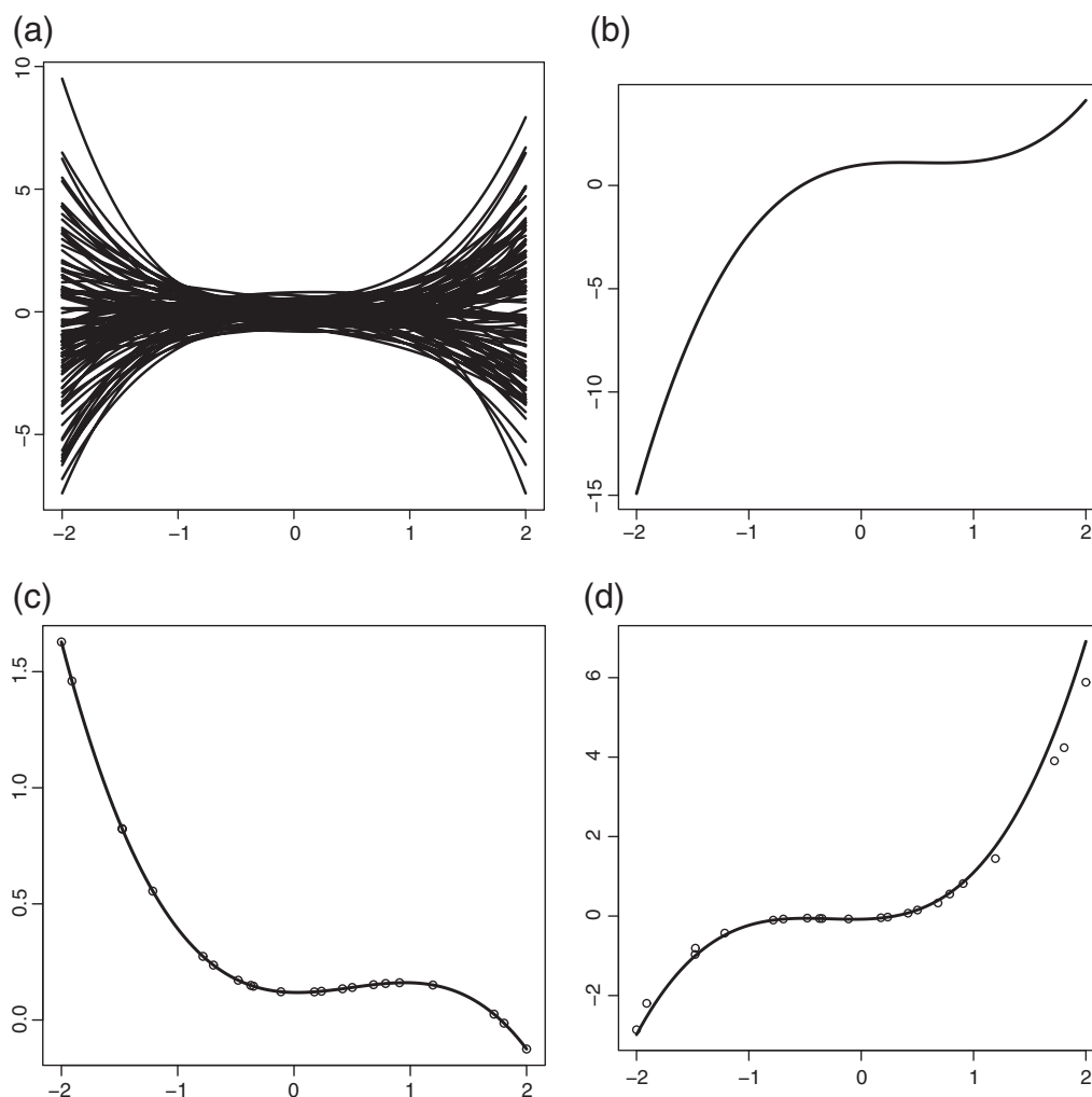
Fig. 8. Case II. (a) Sample of n = 100 simulated curves. (b) Simulated functional parameter. (c) (d) Cubic spline approximation of two specific sampled curves.
