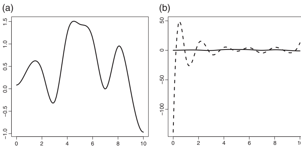
Fig. 2. Case I. (a) Simulated parameter function. (b) Simulated parameter function (solid line) and its estimation in terms of B-splines using least squares criterion.
