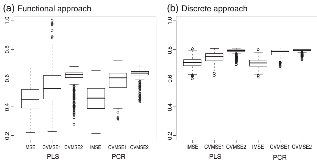
Fig. 5. Case I (IMSE). Box plots for the distribution of the integrated mean squared error (IMSE) for the functional and discrete PLS and PCR models selected with the three criteria considered (IMSE, CVMSE1 and CVMSE2).
