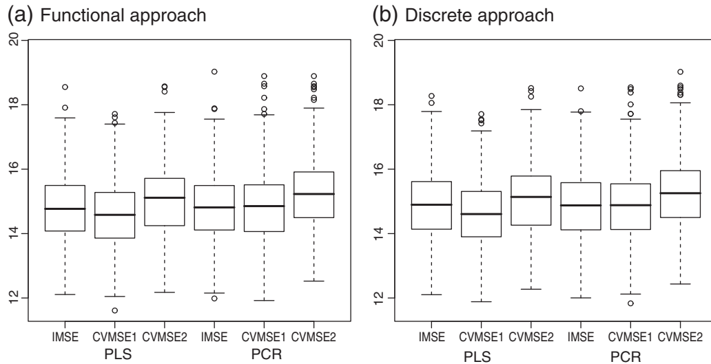
Fig. 6. Case I (CVMSE). Box plots for the distribution of the cross-validation mean squared error (CVMSE) for the functional and discrete PLS and PCR models selected with the three criteria considered (IMSE, CVMSE1 and CVMSE2).
