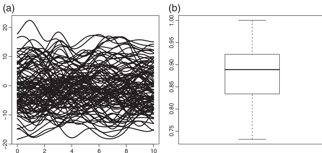
Fig. 1. Case I. (a) Sample of n = 100 simulated curves. (b) Box and Whisker plot of correlation between columns of A\Phi matrix.
