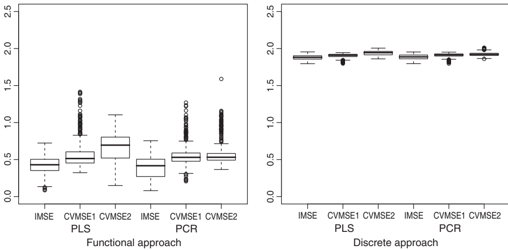
Fig. 10. Case II (IMSE). Box plots for the distribution of IMSE for the functional and discrete PLS and PCR models selected with the three considered criteria (IMSE, CVMSE1 and CVMSE2).
