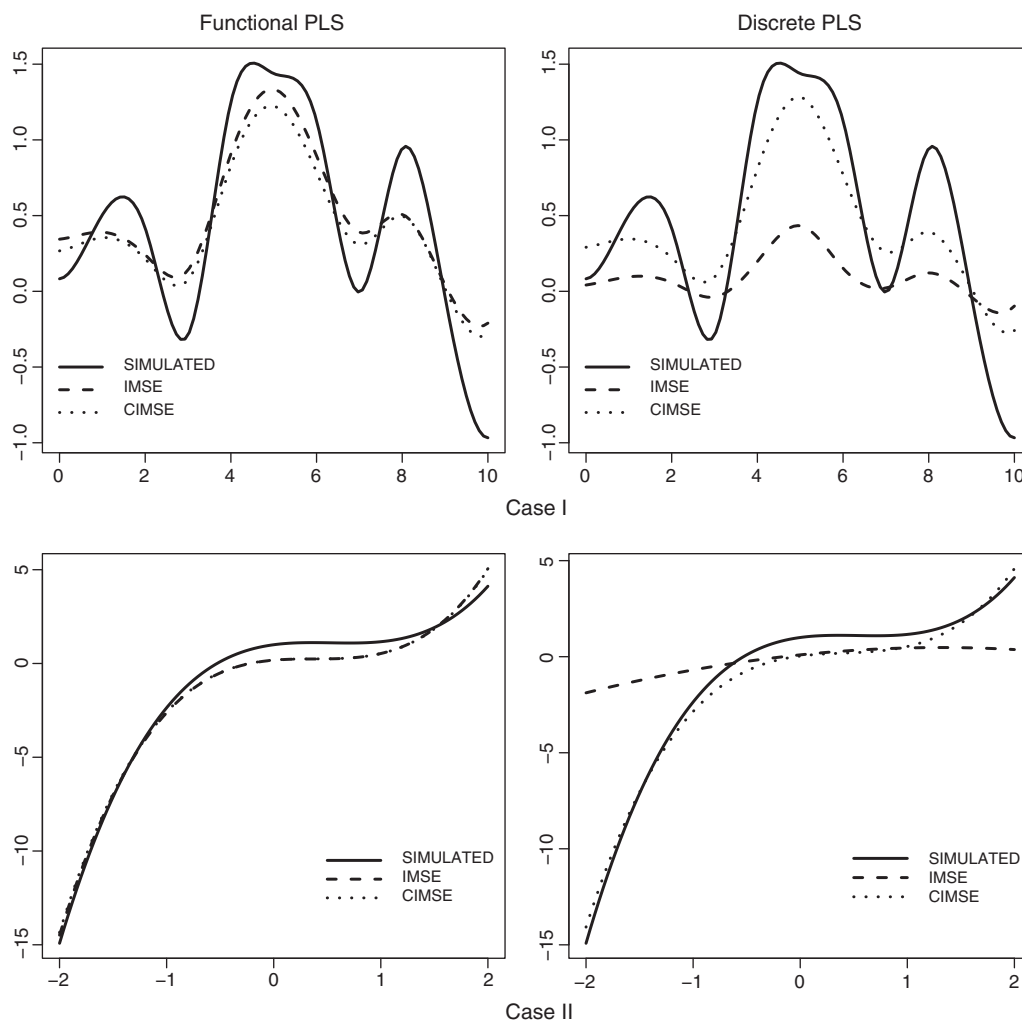
Fig. 13. Simulated parameter function and the mean of its optimum estimations with the two criteria based on the integrated mean squared error (IMSE and CIMSE) on N = 500 repetitions.
