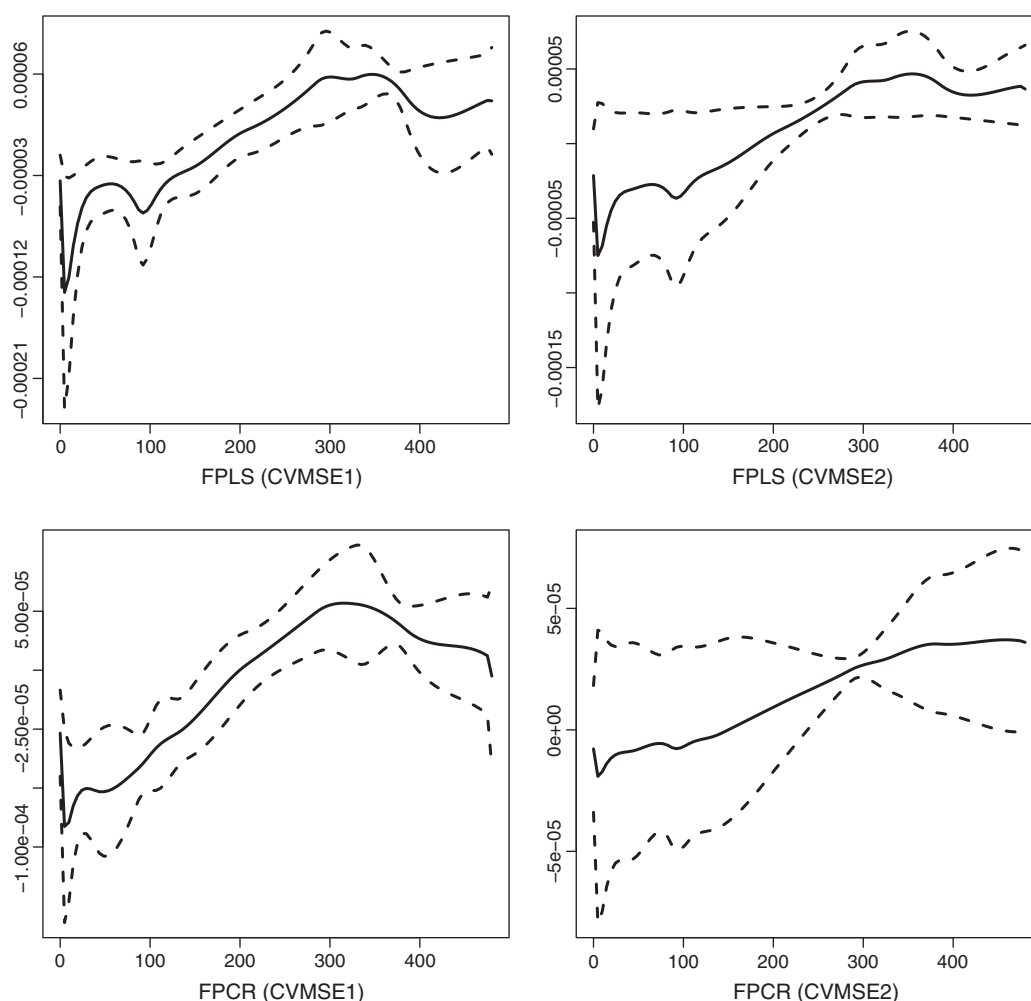
Fig. 15. Kneading data. Average of the optimum functional parameters (solid line) together with \pm 2 times the standard deviation (broken line) estimated by using the CVMSE1 and CVMSE2 criteria with the FPLS and FPCR approaches.
