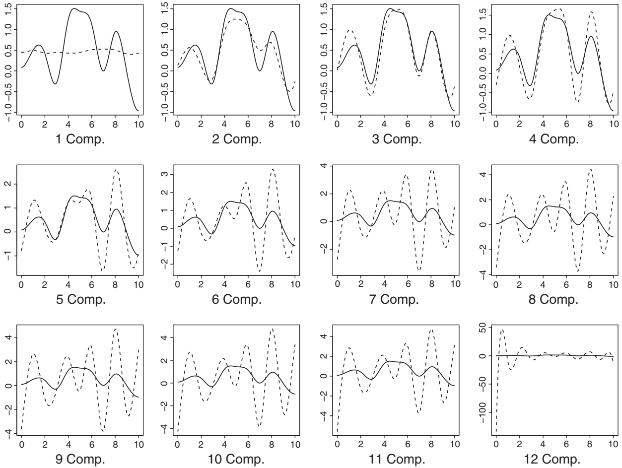
Fig. 3. Case I. Simulated functional parameter (solid line) and its estimations with different numbers of PLS components in the model (dashed).
