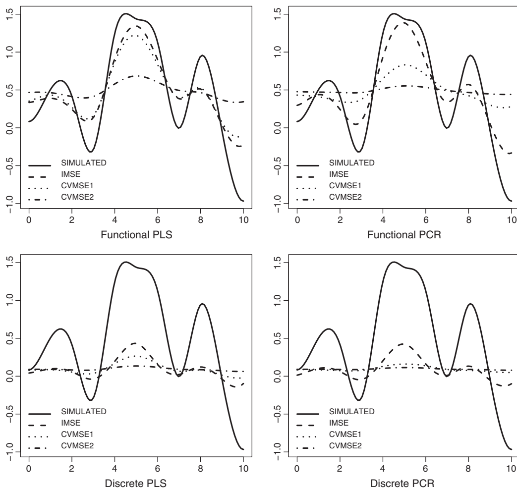
Fig. 7. Case I. Simulated parameter function and the mean of its optimum estimations with the three criteria considered (IMSE, CVMSE1 and CVMSE2) on N = 500 repetitions.
