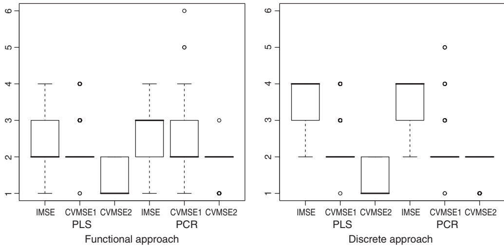
Fig. 9. Case II (NC). Box plots for the distribution of the number of components (NC) for the functional and discrete PLS and PCR models selected with the three considered criteria (IMSE, CVMSE1 and CVMSE2).
