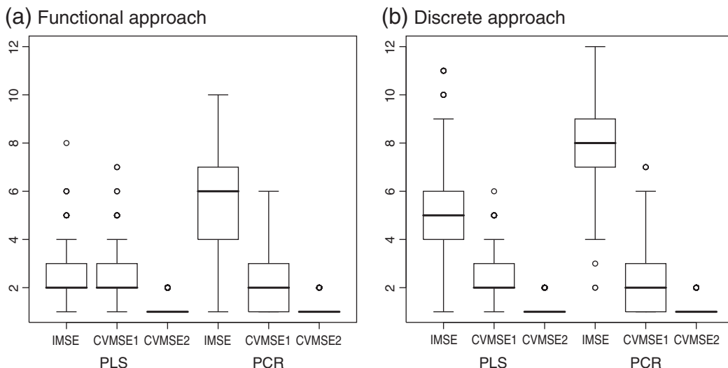
Fig. 4. Case I (NC). Box plots for the distribution of the number of components (NC) for the functional and discrete PLS and PCR models selected with the three criteria considered (IMSE, CVMSE1 and CVMSE2).
