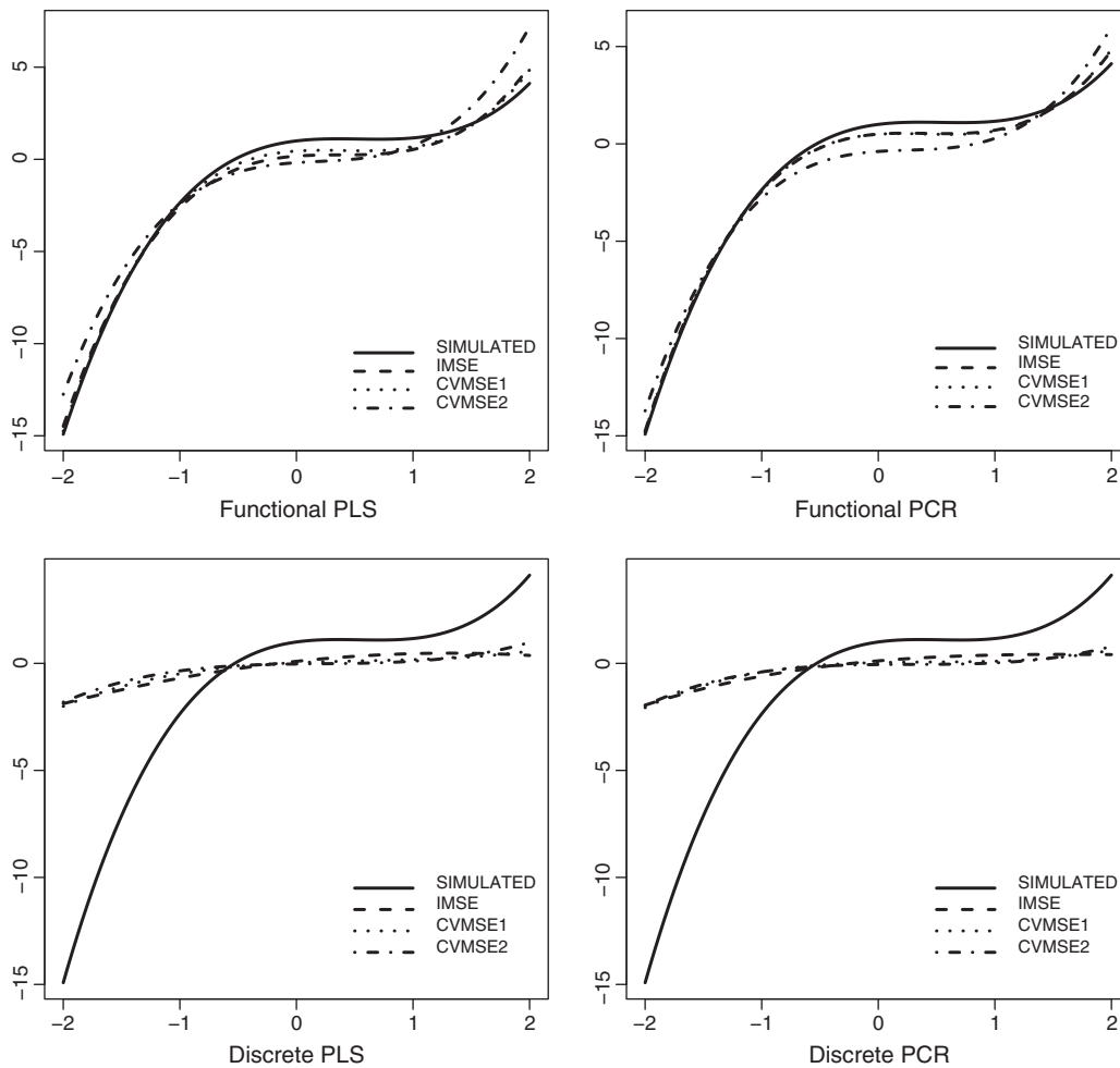
Fig. 12. Case II. Simulated parameter function and the mean of its optimum estimations with the three considered criteria (IMSE, CVMSE1 and CVMSE2) on N = 500 repetitions.
