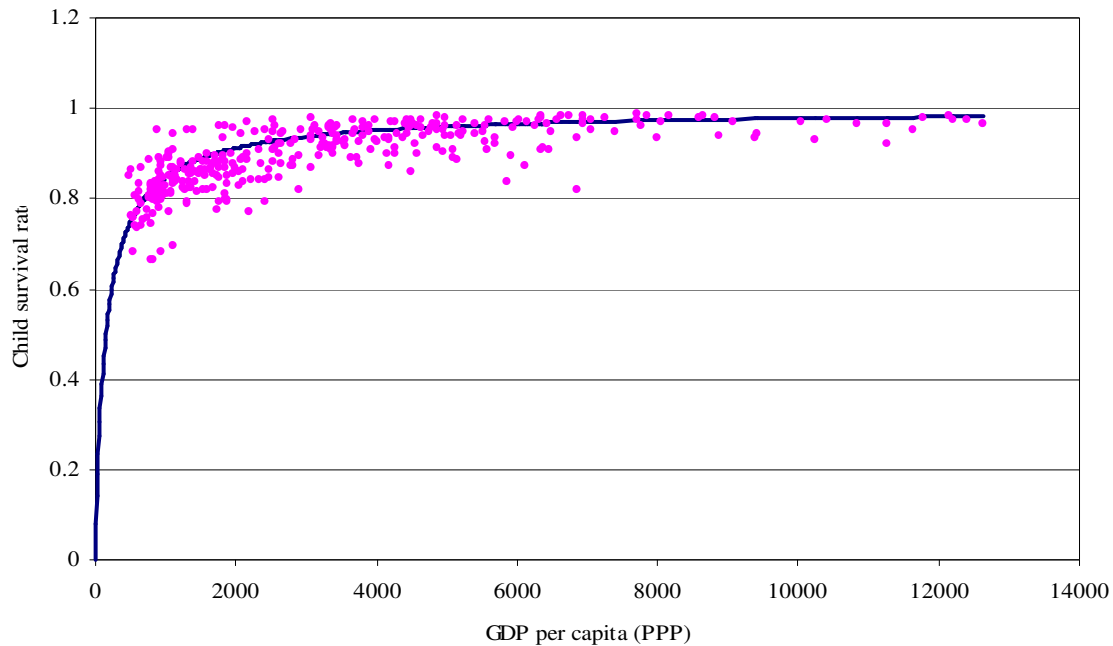
Figure 4: The estimated survival function
