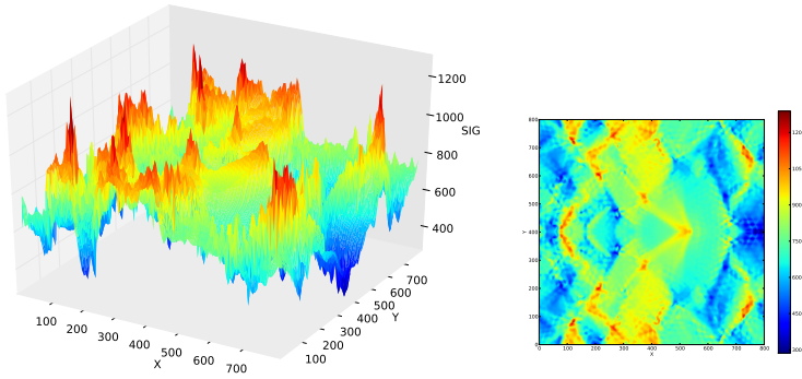
Fig. 8 A realization of the maximal principal stress field \sigma_I
