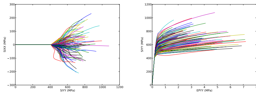
Fig. 6 Mesoscopic behavior in each grain in the X (left) and Y (right) directions
