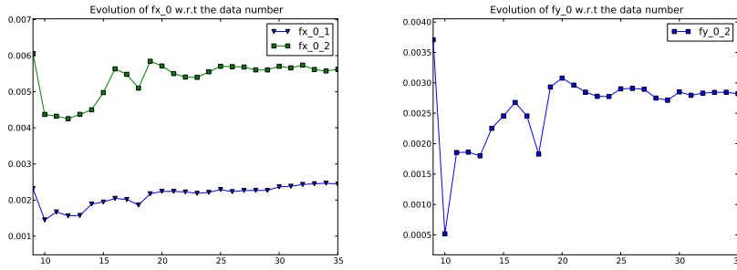
Fig. 16 Case #1: Evolution of the fitted initial frequency in the X, Y directions with respect to the number of realizations K = 8, \dots, 35
