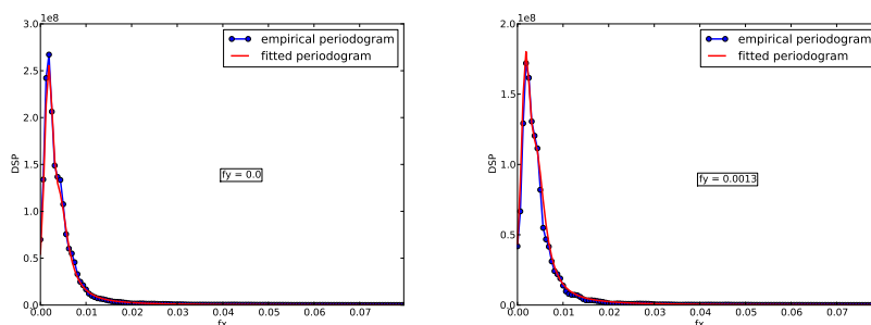
Fig. 22 Case #2: Cut of the periodograms in the X direction
