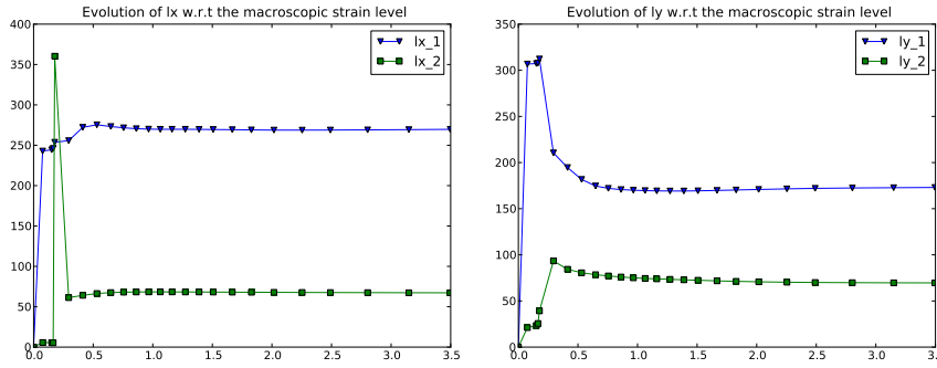
Fig. 28 Case #2: Evolution of the fitted correlation lengths in the X (left) (resp. Y (right)) directions with respect to the load level (macroscopic strain E_{YY} = 0, \dots, 3.5\% )
