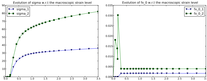
Fig. 27 Case #2: Evolution of the fitted standard deviations (left) with respect to the load level (macroscopic strain E_{YY} = 0., \dots, 3.5\% ) (resp. the initial frequencies f_{(x,y)0}^{(1)} (right))
