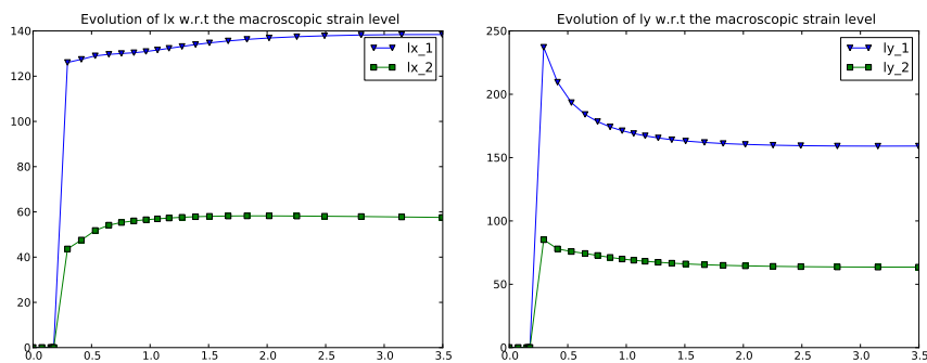
Fig. 18 Case #1: Evolution of the fitted correlation lengths in the X, Y directions with respect to the load level (macroscopic strain E_{YY} = 0., \dots, 3.5\% )
