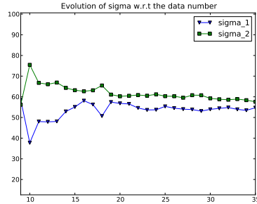
Fig. 14 Case #1: Evolution of the fitted standard deviations with respect to the number of realizations K = 8, \dots, 35
