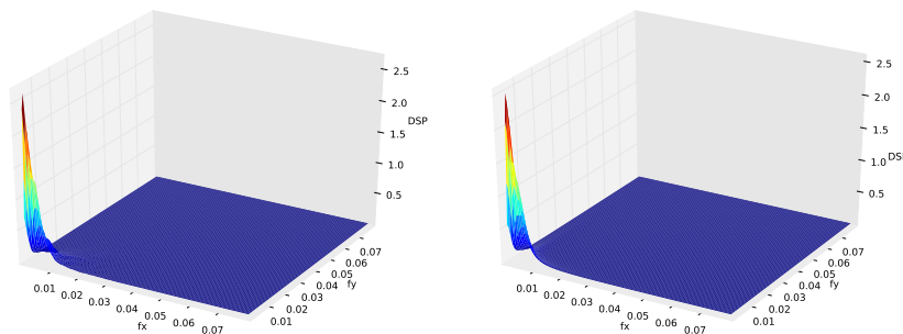
Fig. 21 Case #2: (a) Average empirical periodogram of the stress field at 3.5% macroscopic strain – (b) best fitted periodogram
