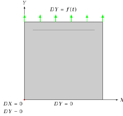
Fig. 4 Boundary conditions used for simulating the tensile test
