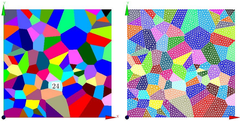
Fig. 3 (a) Two-dimensional polycrystalline aggregate modelling a volume of 16MND5 steel (100 grains) (b) Mesh of the specimen (11,295 nodes)
