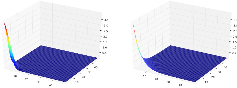
Fig. 1 Gaussian covariance model (left) and Exponential covariance model (right) : \sigma = 2 , l_1 = l_2 = 5
