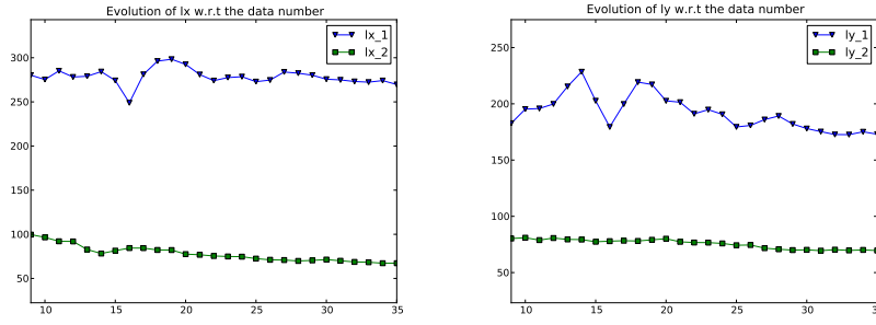
Fig. 26 Case #2: Evolution of the fitted correlation lengths in the X (left) (resp. Y (right)) directions with respect to the number of realizations K = 8, \dots, 35
