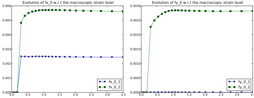
Fig. 19 Case #1: Evolution of the fitted initial frequency in the X, Y directions with respect to the load level (macroscopic strain E_{YY} = 0., \dots, 3.5\% )
