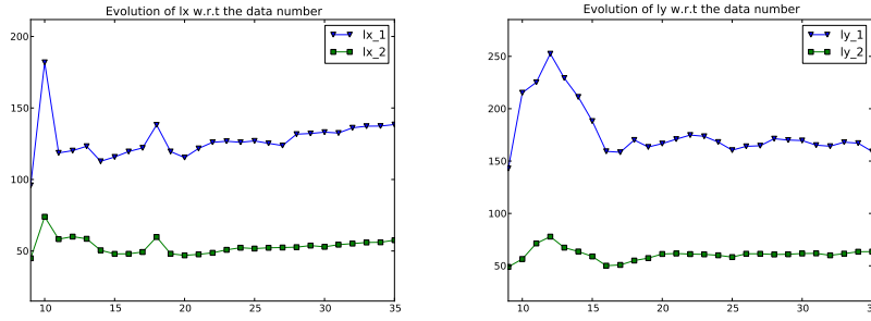
Fig. 15 Case #1: Evolution of the fitted correlation lengths in the X, Y directions with respect to the number of realizations K = 8, \dots, 35
