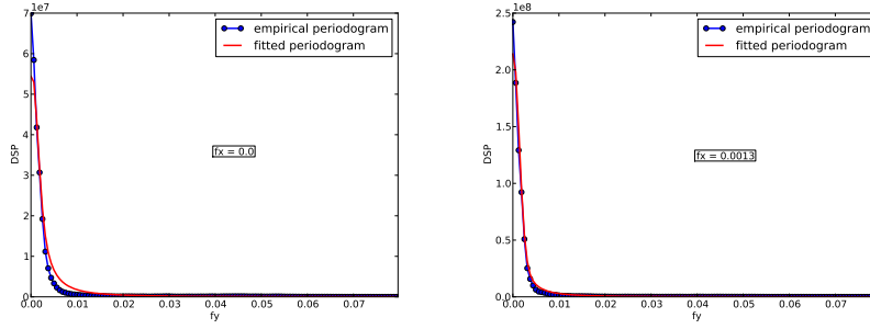
Fig. 23 Case #2: Cut of the periodograms in the Y direction
