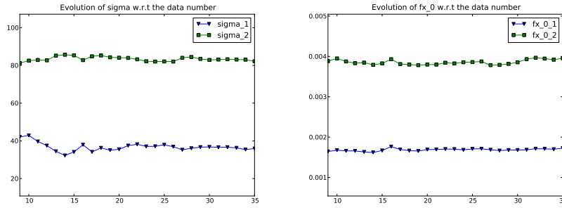
Fig. 25 Case #2: Evolution of the fitted standard deviations and the initial frequencies f_{(x)_0}^{(1,2)} with respect to the number of realizations K = 8, \dots, 35
