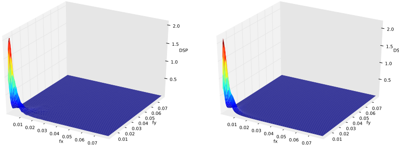
Fig. 10 Case #1: (a) Average empirical periodogram of the stress field at 3.5% macroscopic strain – (b) best fitted periodogram
