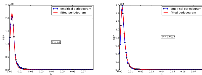
Fig. 11 Case #1: Cut of the periodograms in the X direction
