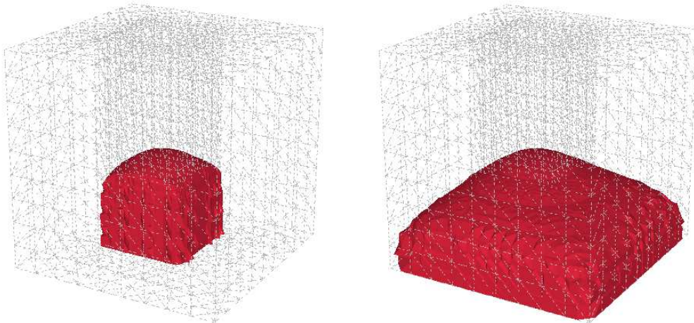
Figure 10: The surfaces u_h(x, t) = 0 and y_h(x, t) = 0 in the (x, t) space. The region below u_h = 0 is the real support of the computed control.
