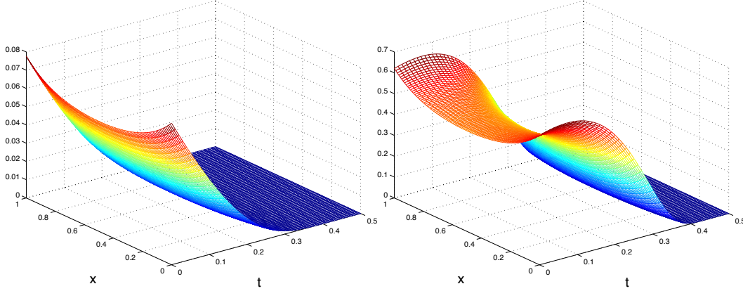
Figure 2: The weights \rho^{-2} and \rho_0^{-2} defined by (10), with \beta_0 = \beta_{0,1/2} defined by (55), K_1 = 0.1 and K_2 = 2\|\beta_0\|_{L^\infty(0,1)} .
