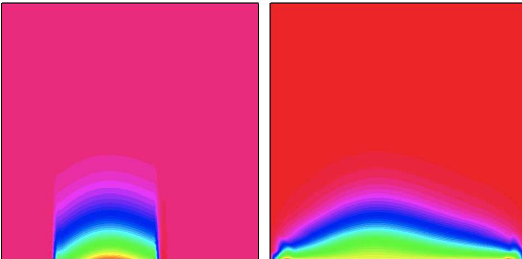
Figure 9: Control and state iso-lines at x_1 = 0.44 . Minimal and maximal values for u_h : -1.26 \times 10^3 , 1.17 \times 10^2 . Minimal and maximal values for y_h : -2.84 \times 10^3 , 3.70 \times 10^1 .
