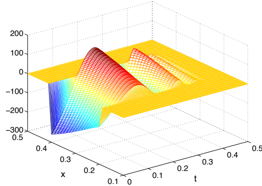
Figure 6: \omega = (0.2, 0.4) - y_0(x) = e^{-300(x-3/4)^2} . The control v_h on (0.1, 0.5) \times (0, T)
