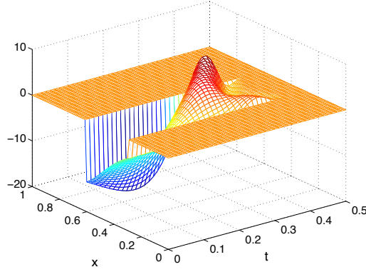
Figure 4: \omega = (0.3, 0.6) . The control v_h .
