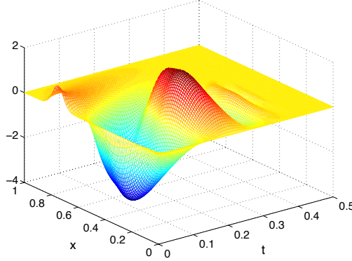
Figure 5: \omega = (0.2, 0.4) - y_0(x) = e^{-300(x-3/4)^2} . The state y_h on Q_T
