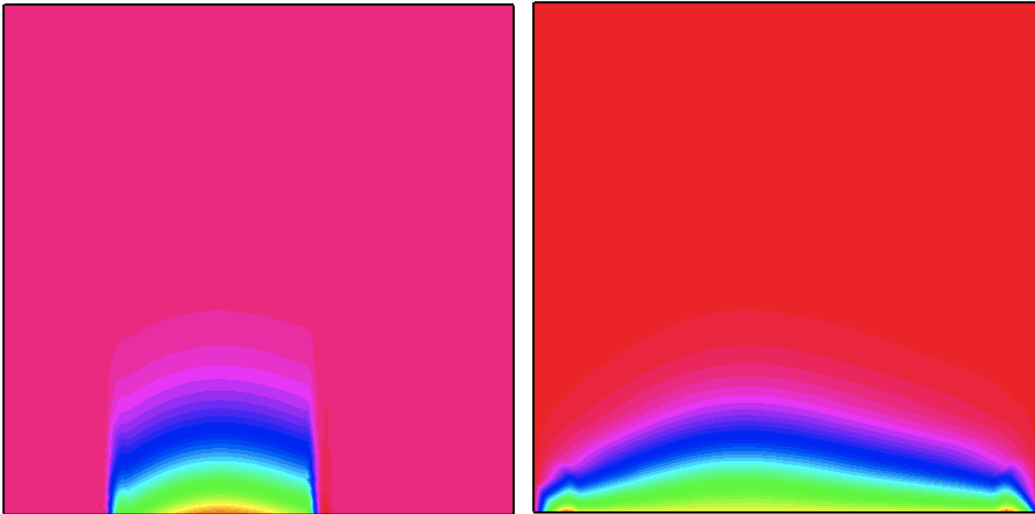
Figure 8: Control and state iso-lines at x_1 = 0.28 . Minimal and maximal values for u_h : -9.89 \times 10^2 , 9.45 \times 10^1 . Minimal and maximal values for y_h : -2.84 \times 10^3 , 3.70 \times 10^1 .
