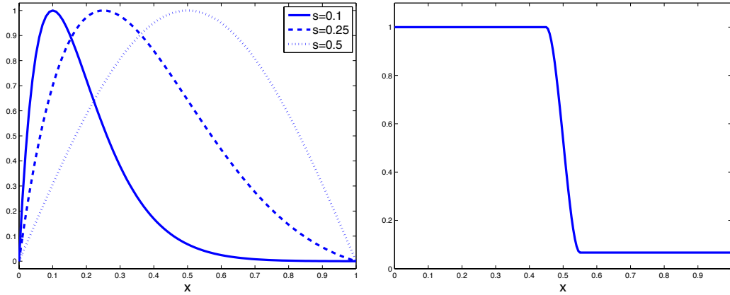
Figure 1: Left: The function \beta_{0,s} on (0,1) for s = 0.1 , s = 0.25 and s = 0.5 . Right: The non-constant C^1 diffusion coefficient a used in Section 4.2 (first case).
