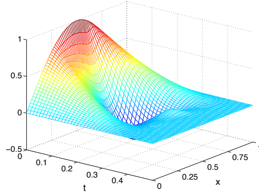
Figure 3: \omega = (0.3, 0.6) . The state y_h .
