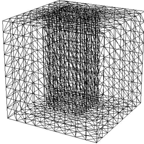
Figure 7: The space-time domain and the mesh: 2 800 vertices. Total number of unknowns (the values of m_h , r_h and \lambda_h at the nodal points, see (63)): 6\,846 \times 3 = 20\,538 .
