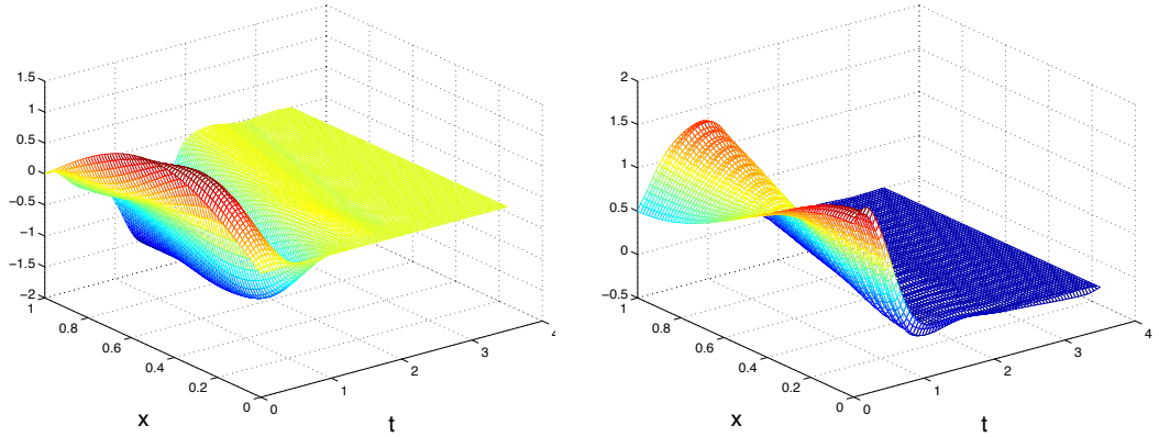
FIGURE 8. \beta = 0 : Minimizer y_{1h} ( left ) and y_3 ( right ) over q_T .
