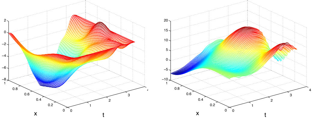
FIGURE 13. \beta = 0 : Minimizer y_{1h} ( left ) and y_{3h} ( right ) over q_T .
