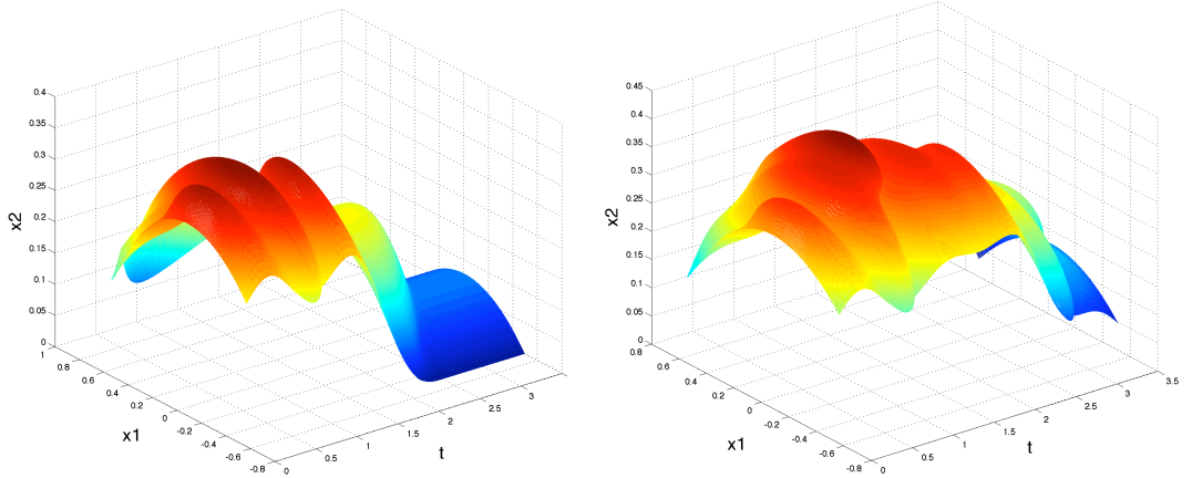
FIGURE 4. Evolution of the controlled ( left ) and uncontrolled ( right ) arch in the plane (O, x_1, x_2) vs. t \in (0, T) .
