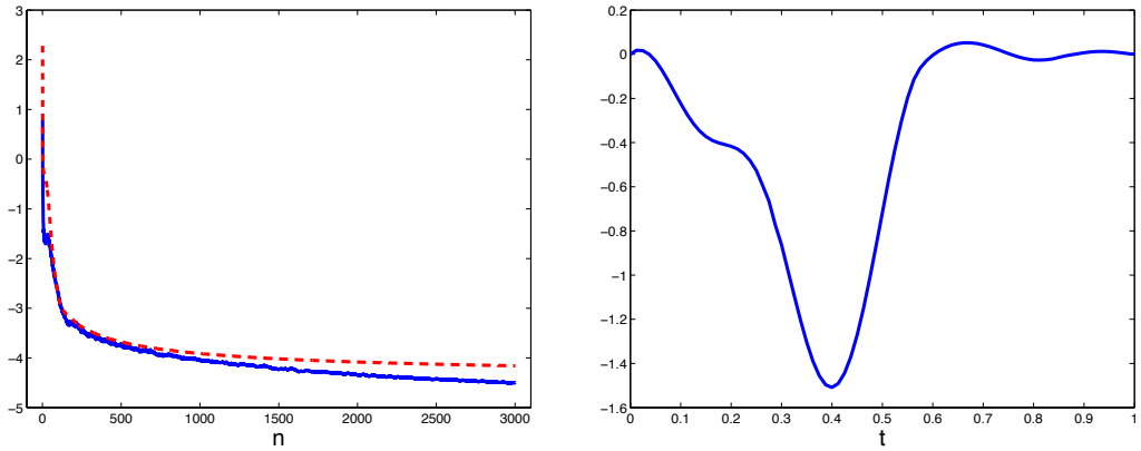
FIGURE 7. \beta = 0 : T = 3.5 , \Delta x = \Delta t = 1/80 - Left : \log_{10} of E_h(\mathbf{y}_h^n) ( dashed line ) and \log_{10}(\|\mathbf{g}_h^n\|_{\mathcal{A}_0}) ( full line ) vs. the iteration n of the conjugate gradient algorithm ; Right : Trace y_{1h}(\xi = 1, t) vs. t \in (0, T)
