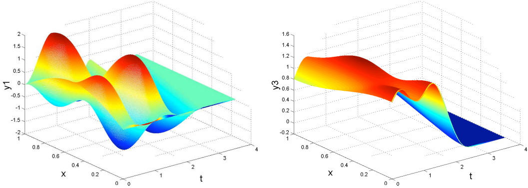
FIGURE 2. Controlled solution \mathbf{y} = (y_1, y_3)
