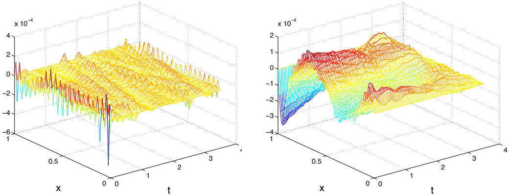
FIGURE 14. \beta = 0 : Minimizer y_{1h} ( left ) and y_{3h} ( right ) over q_T .
