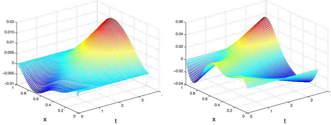
FIGURE 11. \beta = 1 ; Minimizer u_{1h} ( left ) and u_{3h} ( right ) over q_T .
