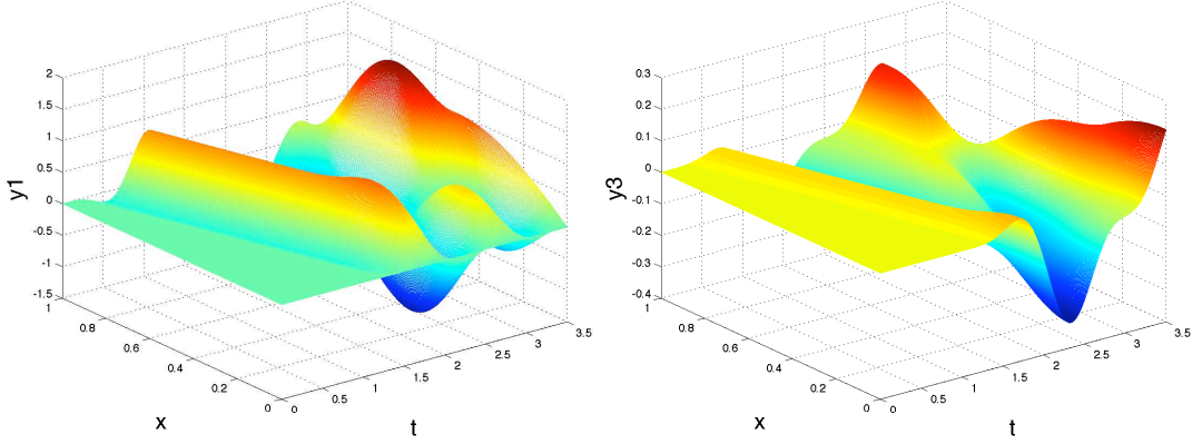
FIGURE 6. Evolution of the controlled component y_1 vs. t ( left ) and corresponding evolution of the component y_3 ( right ), starting from (\mathbf{0}, \mathbf{0}) .
