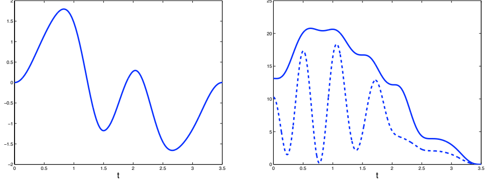
FIGURE 1. Left: Control of minimal L^2(\Sigma_T) -norm v vs. t \in (0, T) ; Right: Energy (solid line) and kinetic energy (dashed line) vs. t \in (0, T) .
