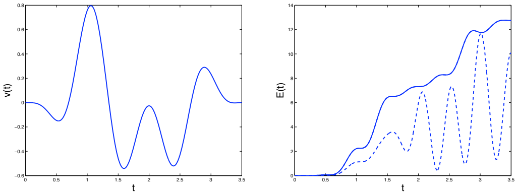
FIGURE 5. left : Partial control v vs. t \in (0, T) ; right : Energy (solid line) and kinetic energy (dashed line) vs. t \in (0, T) .
