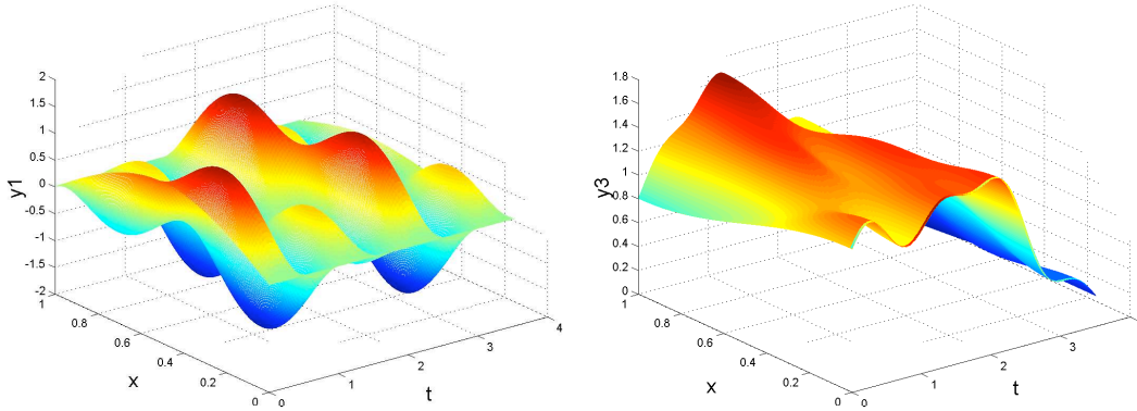
FIGURE 3. Free (uncontrolled) solution \mathbf{y} = (y_1, y_3)
