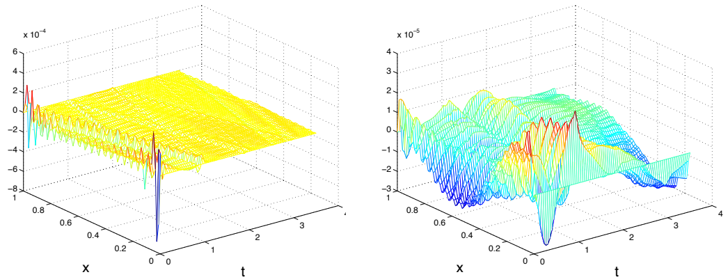
FIGURE 9. \beta = 0 ; Minimizer v_{1h} ( left ) and v_3 ( right ) over q_T .
