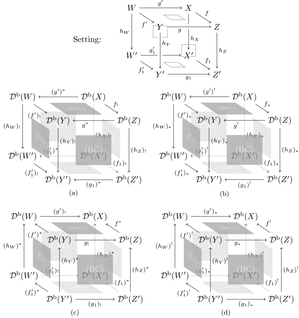
FIGURE B.8. Base change and iterated composition
