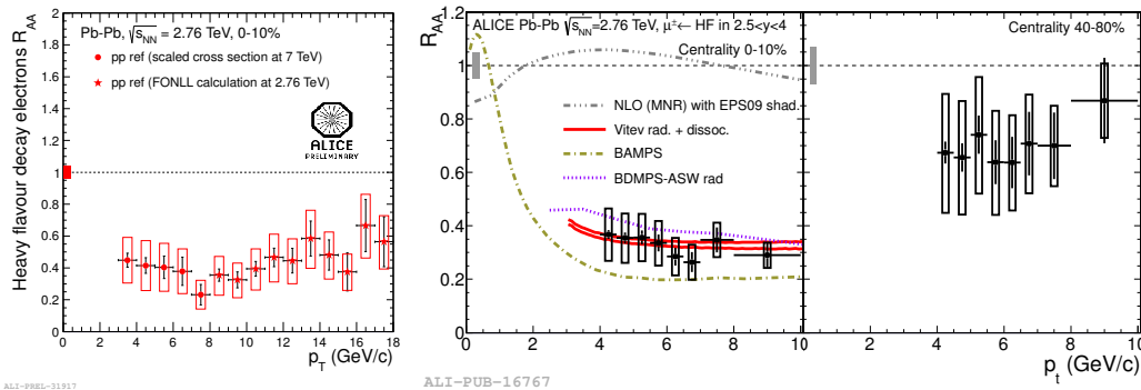
Figure 2. R_{AA} of electrons (left) and muons (middle and right) from heavy-flavour decays for different centrality classes. The statistical (bars), systematic (empty boxes) and normalization (filled boxes) uncertainties are shown. R_{AA} of muons from heavy-flavour decays [10] is compared to models including only shadowing and to models implementing in-medium energy loss.
