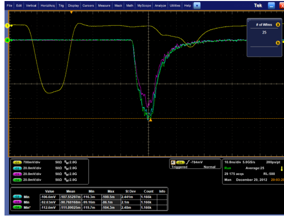
Figure 4.10: Response of 3 of the 16 channels of a Hamamatsu MCPPMT exposed directly to a fast optical pulse (yellow pulse). This led pulse is 20 ns in length.
