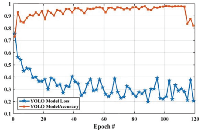
Figure 13: The YOLO model performance is based on training data
