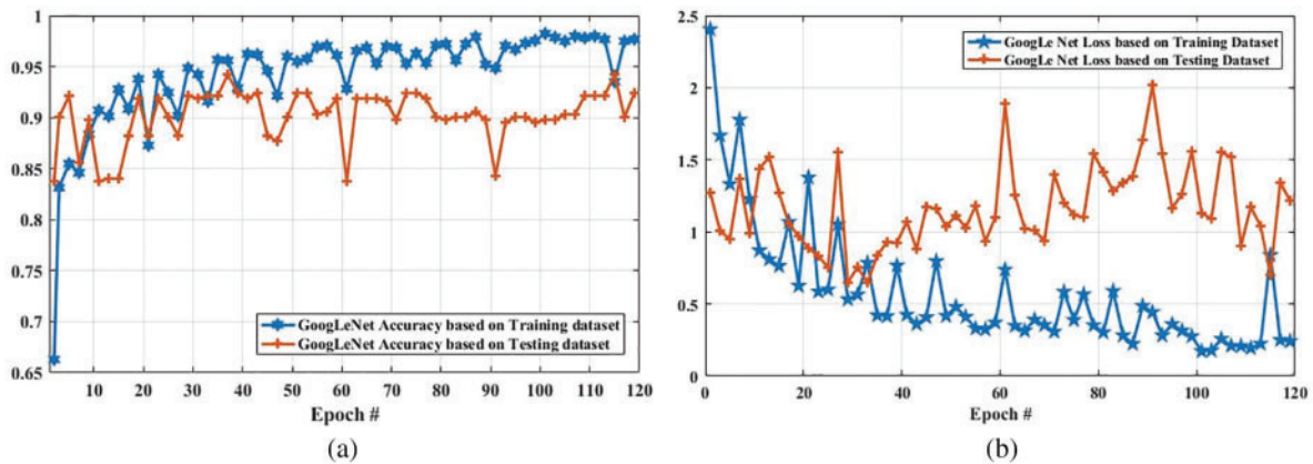
Figure 9: Accuracy and loss comparison of GoogLeNet model based on training and testing dataset. (a) Depicts the accuracy of GoogLeNet model based on training and testing dataset, and (b) illustrates the loss of GoogLeNet model based on training and testing dataset
