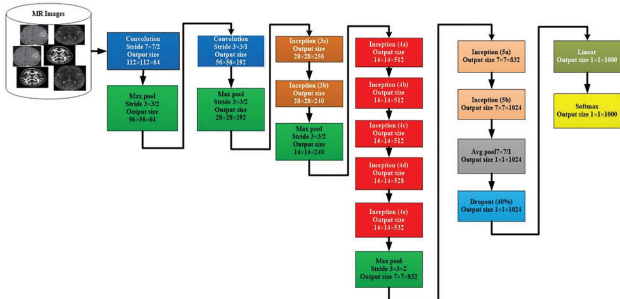
Figure 4: GoogLeNet model for image classification
