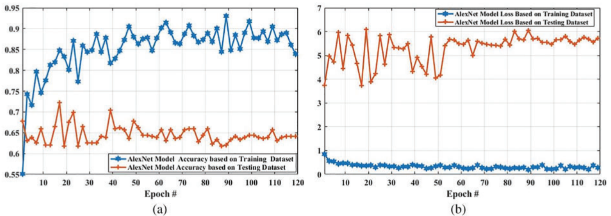
Figure 12: Accuracy and loss comparison of AlexNet model based on training and testing dataset. (a) Depicts the accuracy comparison of AlexNet model based on training and testing dataset, and (b) presents the loss comparison of AlexNet model based on training and testing dataset
