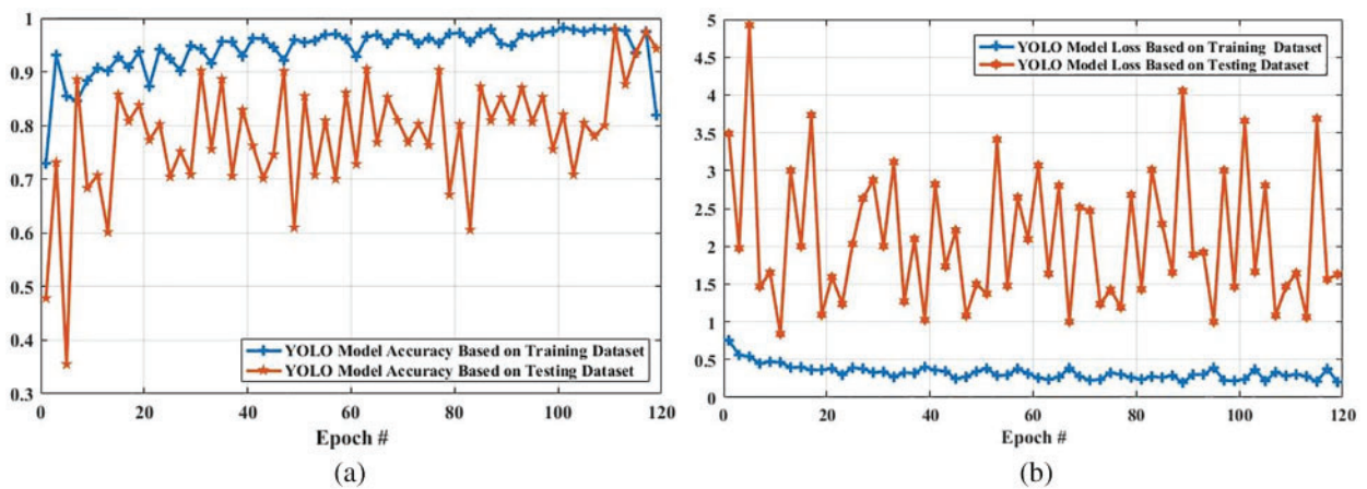
Figure 15: Accuracy and loss comparison of YOLO model based on training and testing dataset. (a) Shows the accuracy comparison of YOLO model based on training and testing dataset, and (b) presents the loss comparison of YOLO model based on training and testing dataset
