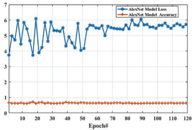
Figure 11: The AlexNet performance is based on the testing dataset
