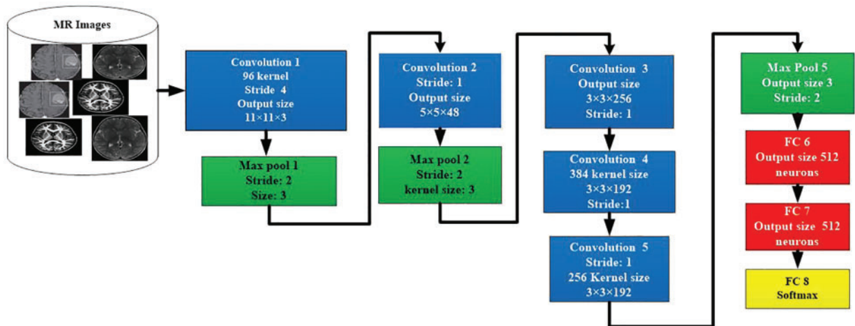
Figure 5: Architecture of AlexNet model for image classification
