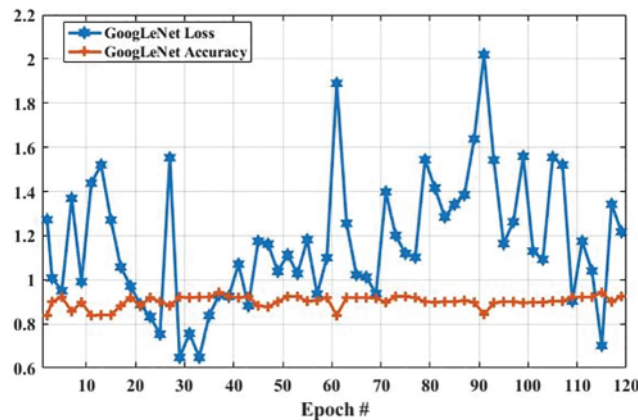
Figure 8: The GoogLeNet performance is based on a testing dataset
