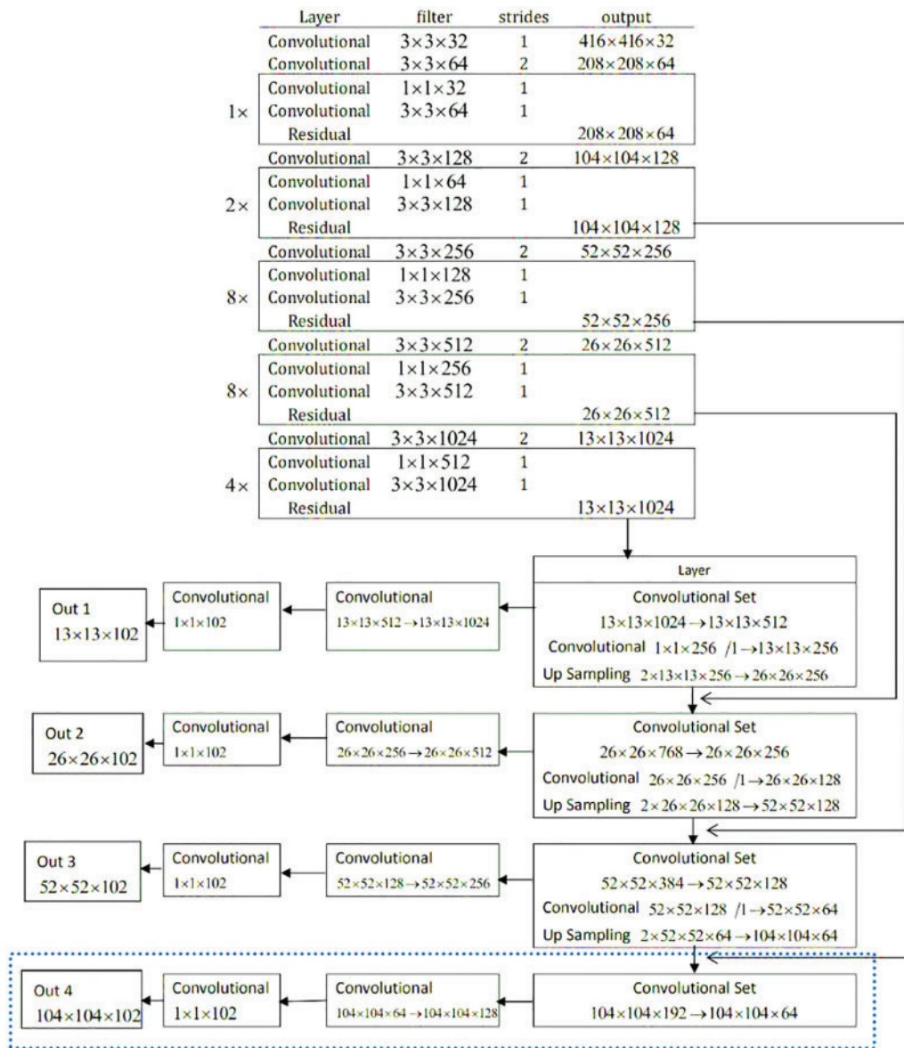
Figure 6: Network architecture of YOLOv3 model for tumor localization
