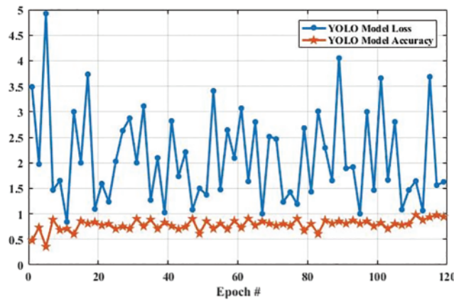
Figure 14: The YOLO model performance is based on testing data
