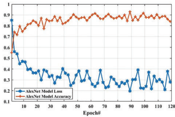
Figure 10: The AlexNet performance is based on the training dataset
