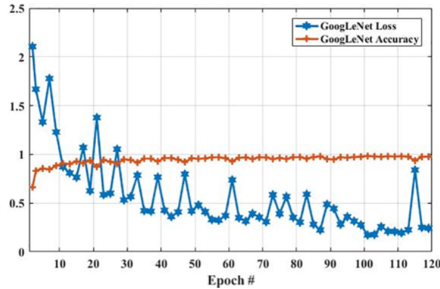
Figure 7: The GoogLeNet performance is based on the training dataset
