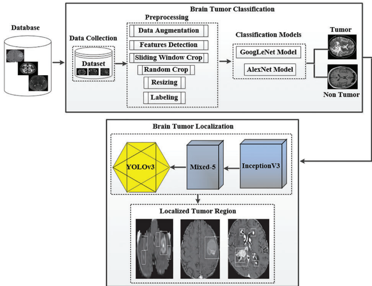
Figure 1: The proposed framework of tumor classification and localization
