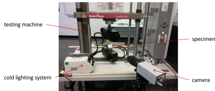
a- Picture of a typical test
