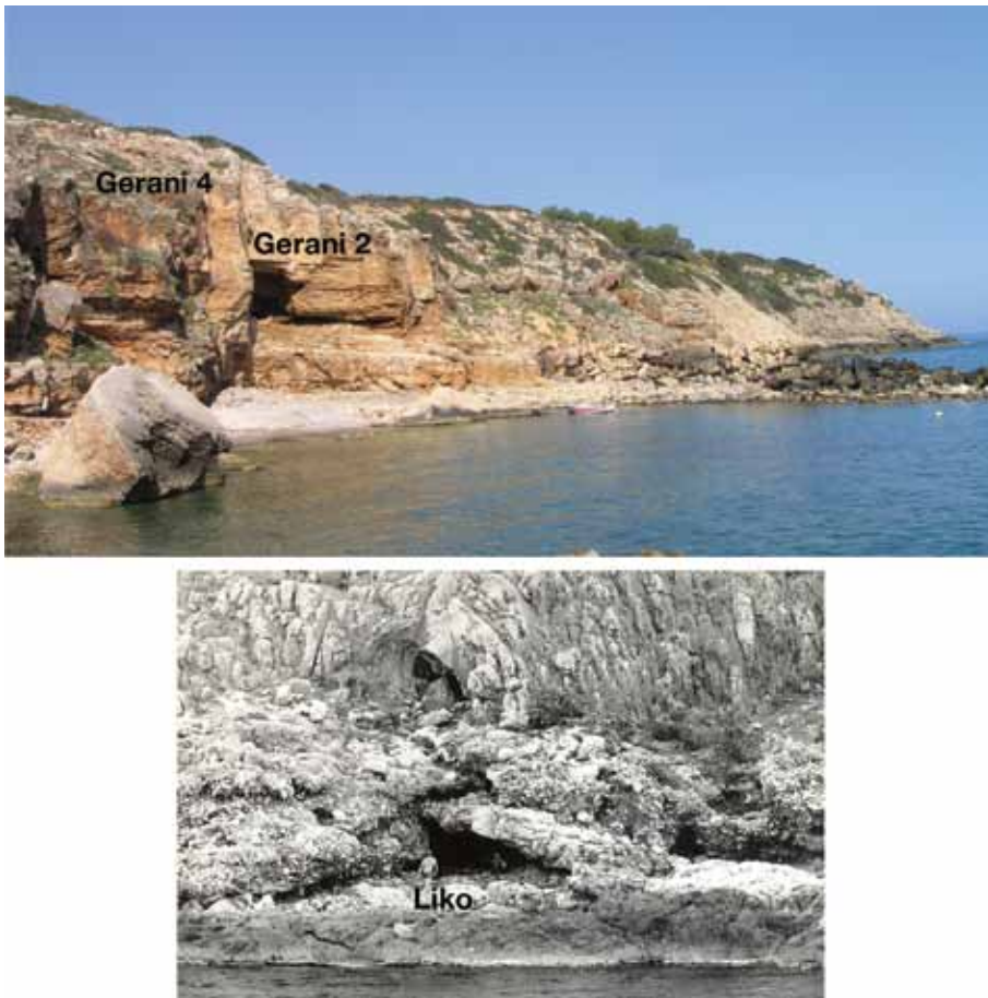
FIG. 2. Views of caves at Gerani (top) and Liko (bottom). These coastal caves are situated in Neogene limestones and contain richly fossiliferous sediments. Photographs: J. de Vos.
