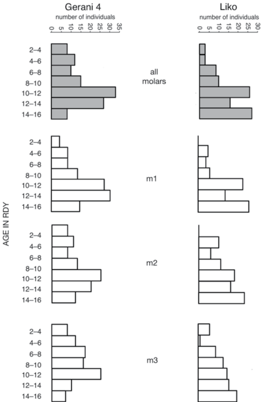
FIG. 4. Mortality profiles (dx) for Candiacerus ropalophorus from Gerani 4 (left) and Candiacerus sp. II from Liko (right), based on age estimations inferred from wear stages of all molars (top histograms) or of m1, m2, or m3 considered singly (other histograms). Although some differences can be observed between the profiles, patterns are essentially the same.
