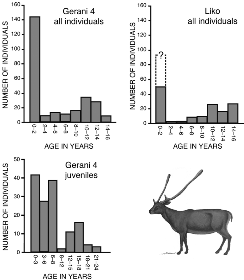
FIG. 6. Mortality profiles (dx) for Candiacervus ropalophorus from Gerani 4 (top left, actual numbers for all ages; bottom left, juveniles only) and Candiacervus sp. II from Liko (top right, all ages). Bottom right, reconstruction of Can. ropalophorus by Alexis Vlachos.
