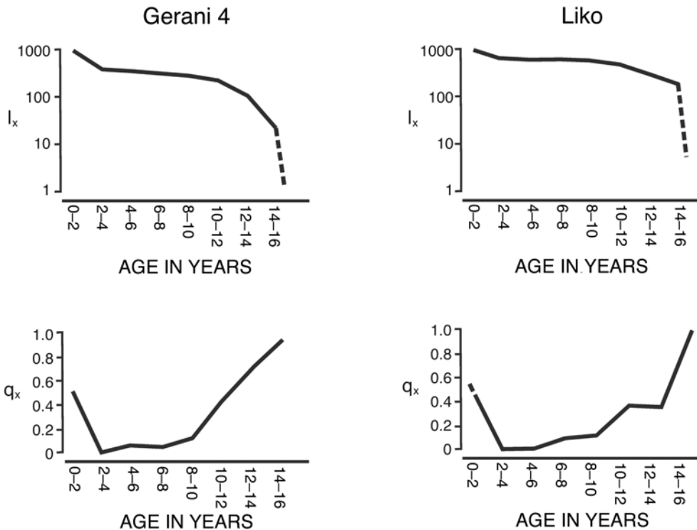
FIG. 7. Survivorship curves ( l_x ) and mortality rates ( q_x ) (top and bottom, respectively) for Candiacervus ropalophorus (Gerani 4) and Candiacervus sp. II (Liko).
