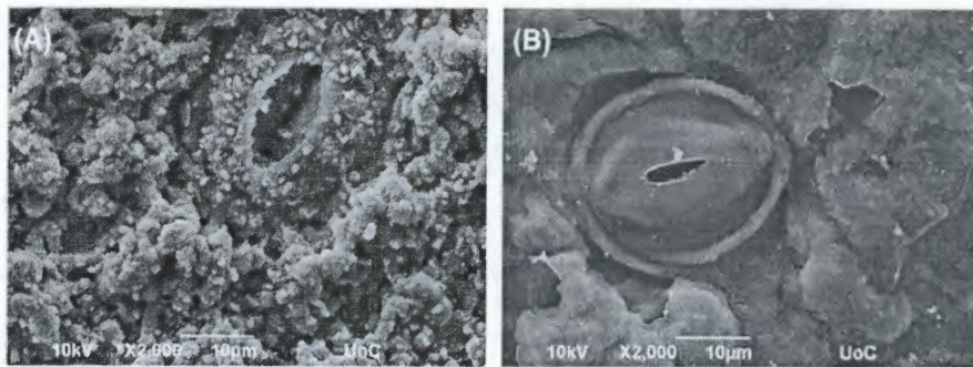
Fig. 3. Scanning electron micrographs of abaxial leaf surface of (A) Arbutus andrachne and (B) Arbutus unedo showing in detail the topography and microsculpturing of epicuticular waxes (magnification 2000 \times ).
