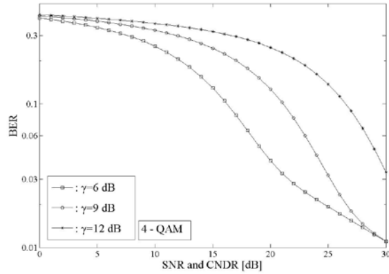
Figure 1. BER estimation for the 4-QAM OFDM system.
