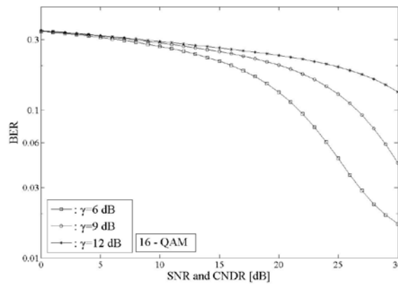
Figure 2. BER estimation for the 16-QAM OFDM system.
